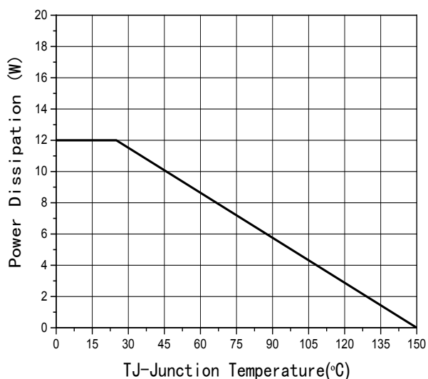
Fig7 Power De-rating
