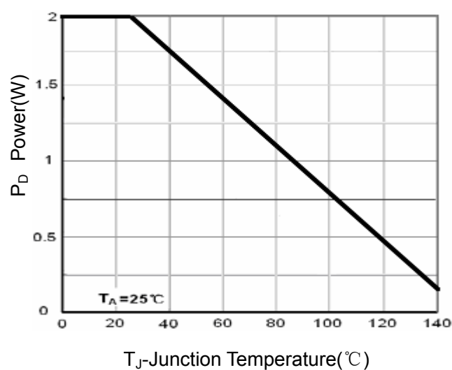
Figure 8 Power Dissipation
