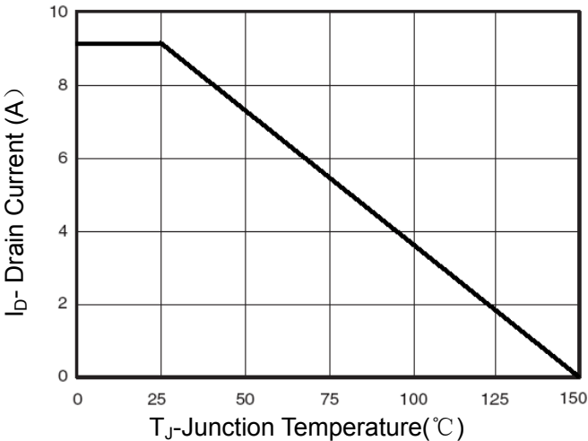
Figure 4 Drain Current
