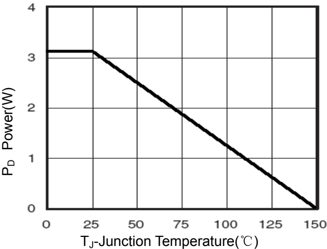
Figure 3 Power Dissipation
