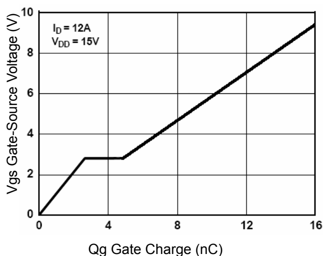
Figure 5 Gate Charge
