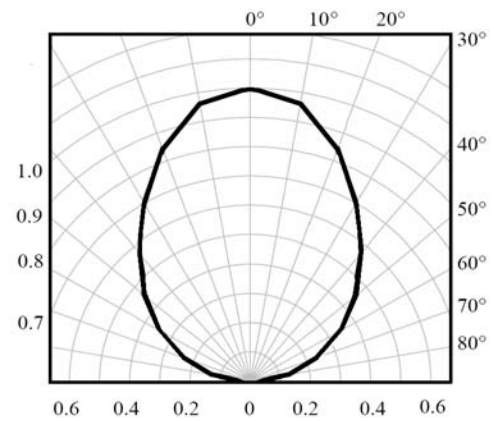
Fig. 4 - Directivity
