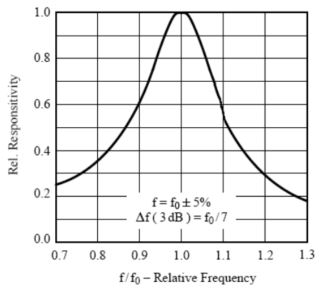
Fig. 3 - Carrier Band pass response
