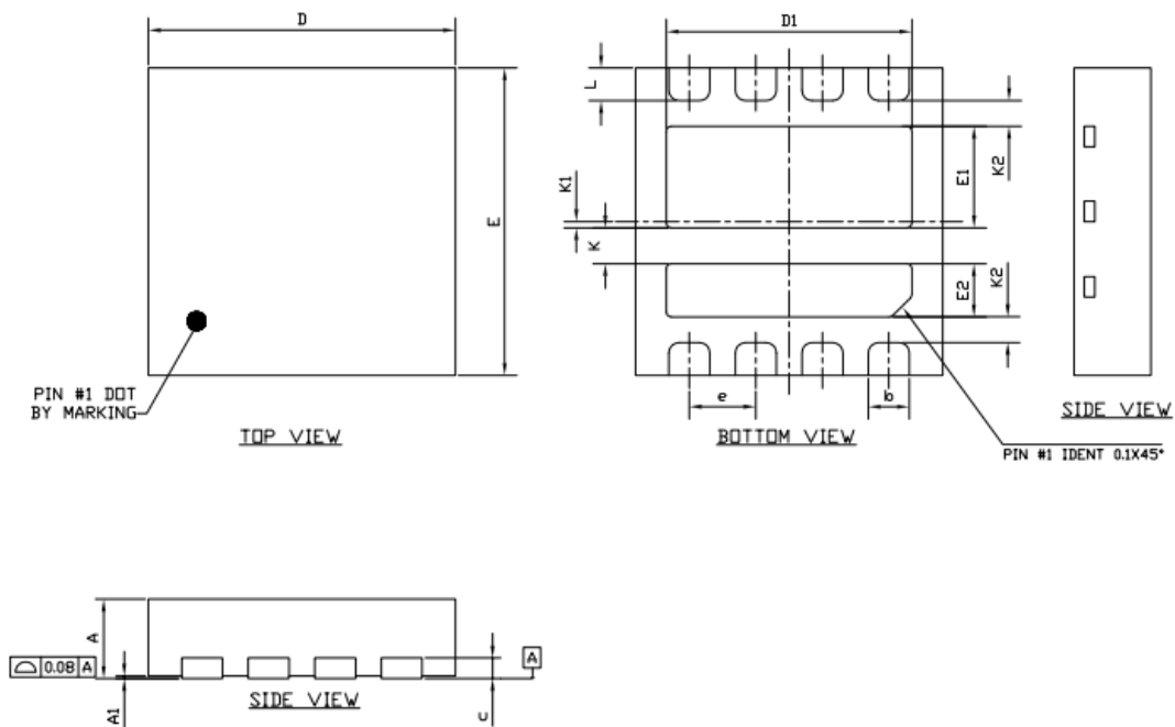
DFN3X3
