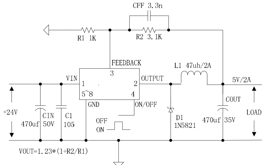
Figure9. HM1509-ADJ System Parameters Test Circuit
