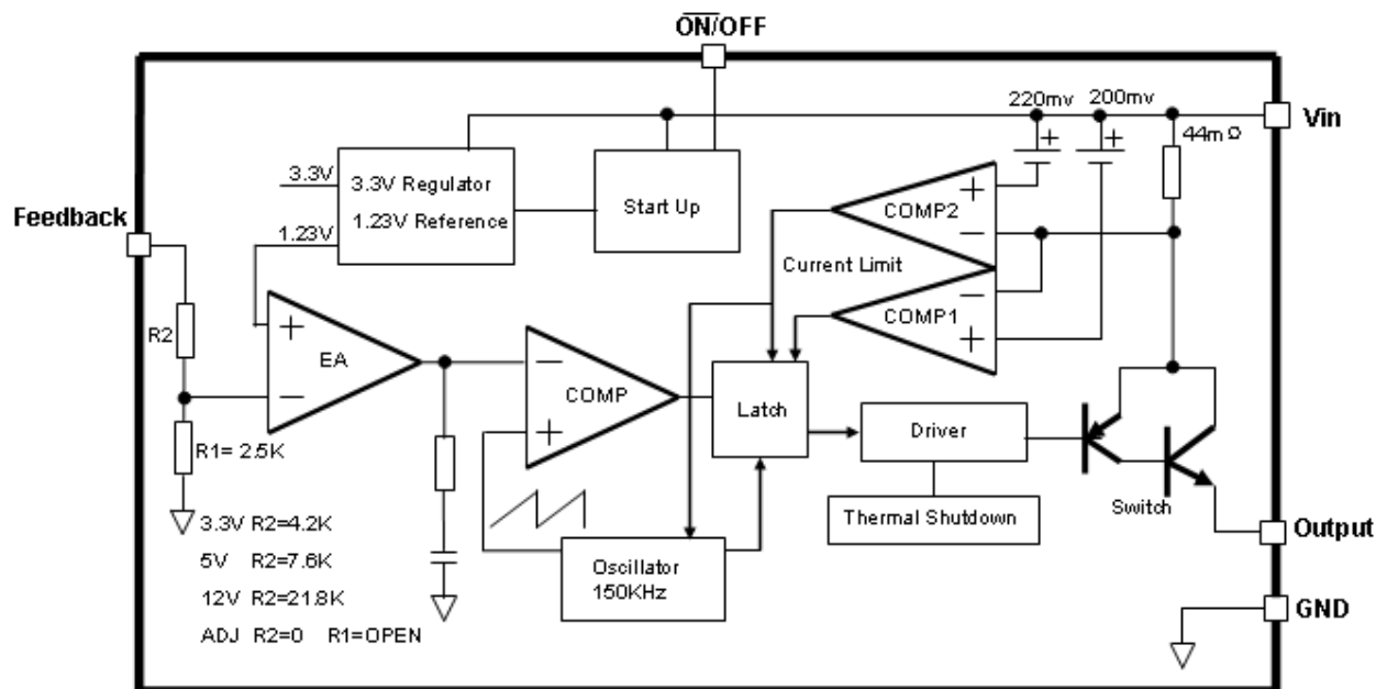
Figure3. Function Block Diagram of HM1509
