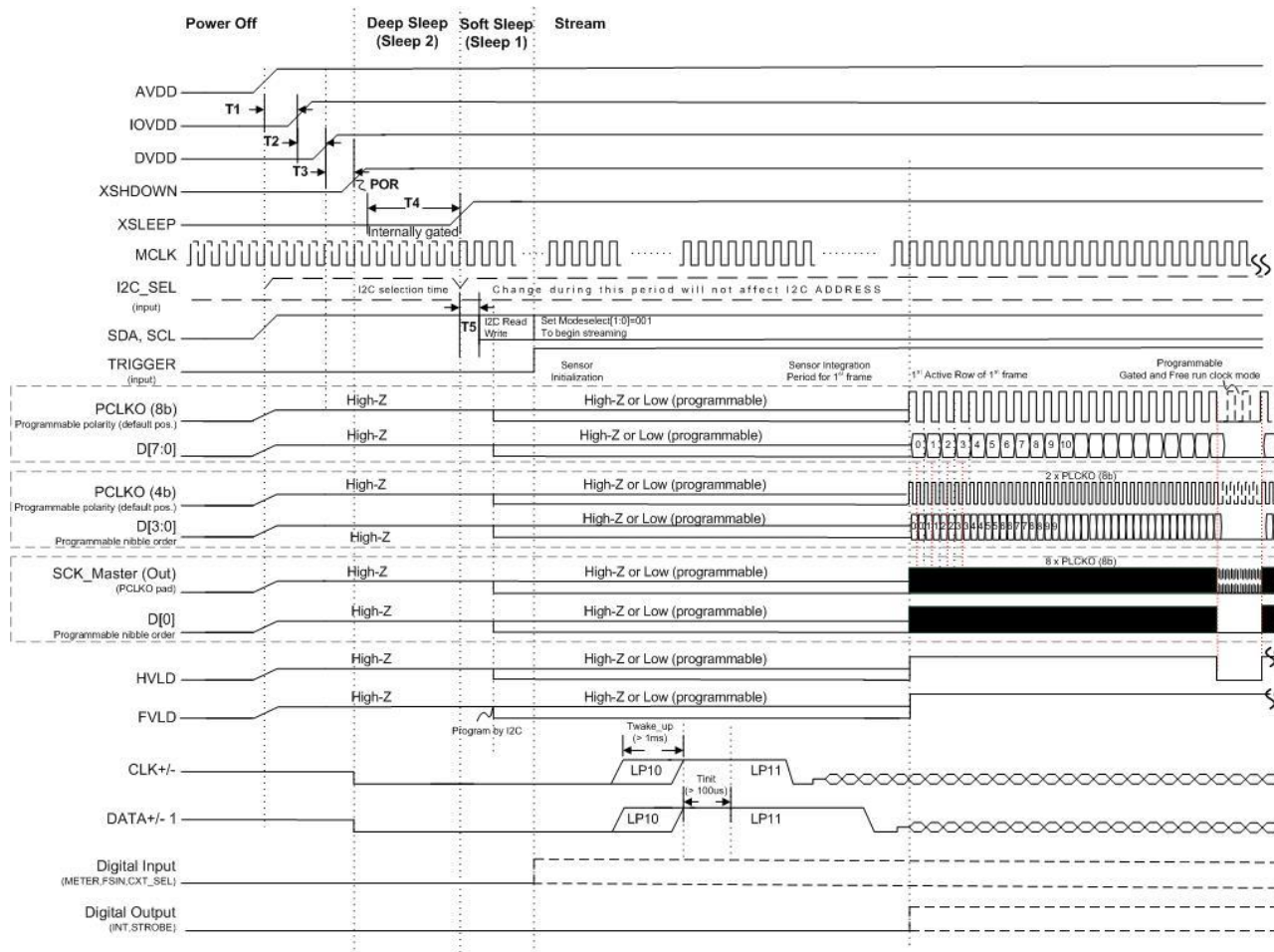
Figure 6.3: Power up sequence
