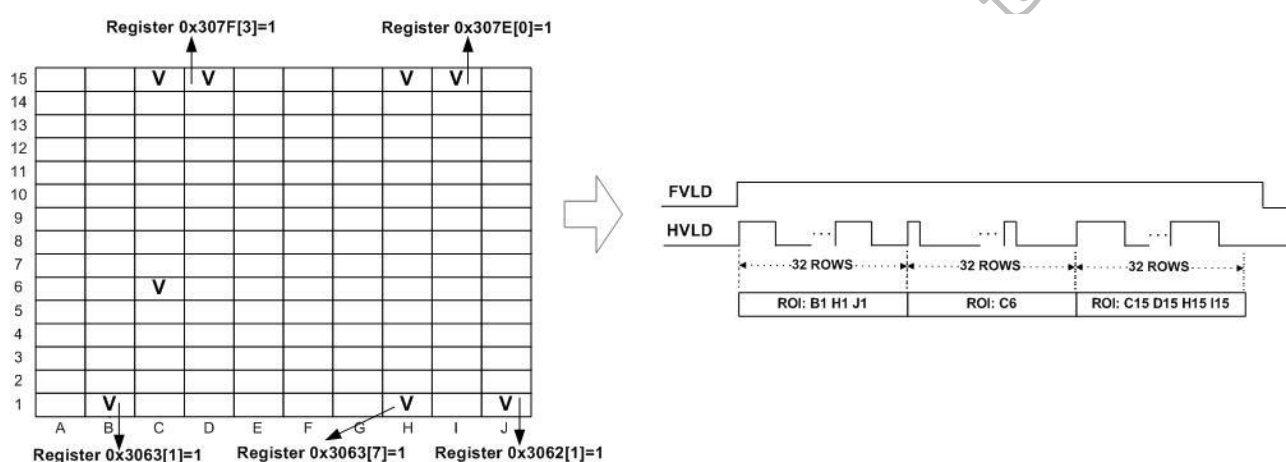
Figure 3.6: VGA ROI window readout with parallel interface
