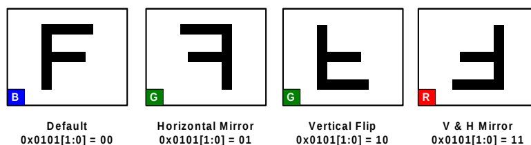
Figure 3.7: Horizontal and vertical mirror readout modes
