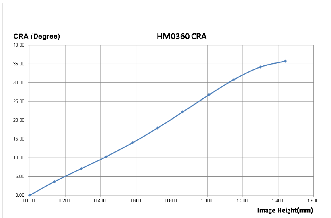
Figure 12.1: Lens CRA profile
