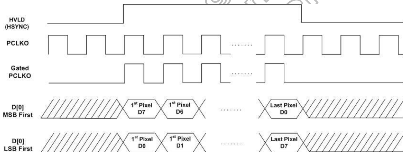
Figure 6.8: Output format on serial data IO interface
