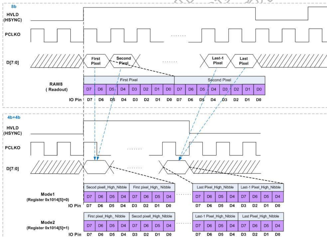
Figure 6.6: Output format on 8-bit data IO interface
