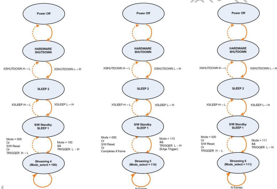
Figure 6.2: State diagram (Hardware pin trigger)
