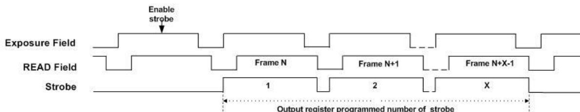
Figure 4.4: Strobe control
