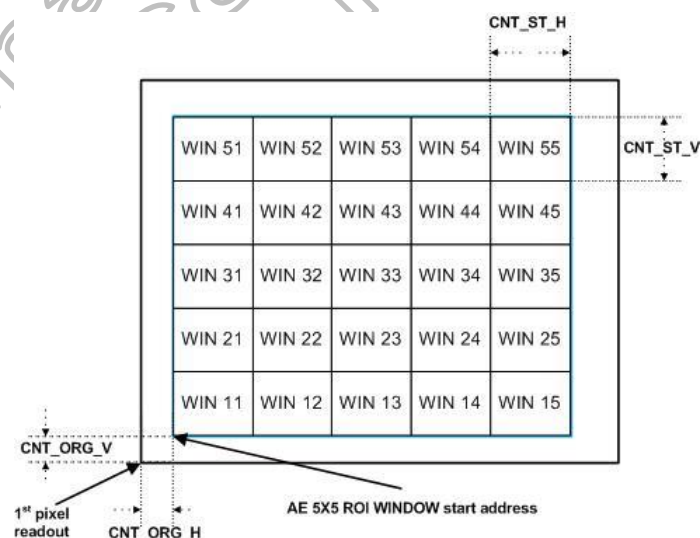
Figure 4.7: AE ROI window
