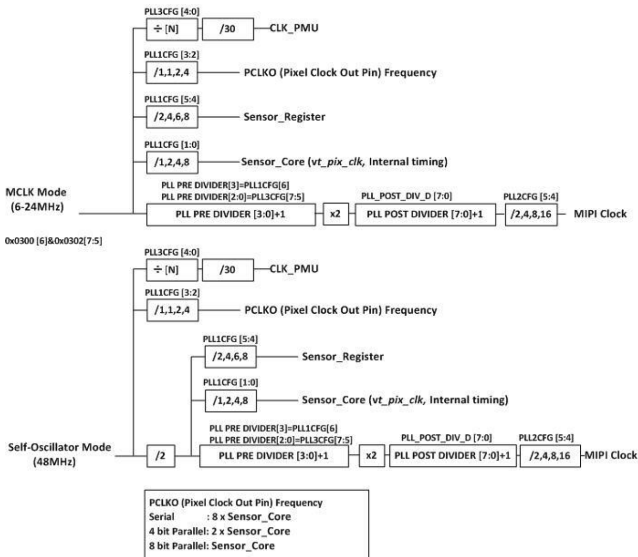
Figure 6.4: Clock dividers
