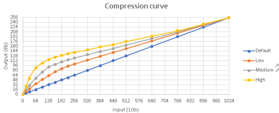
Figure 4.9: Compression curve (input 10b, output 8b)
