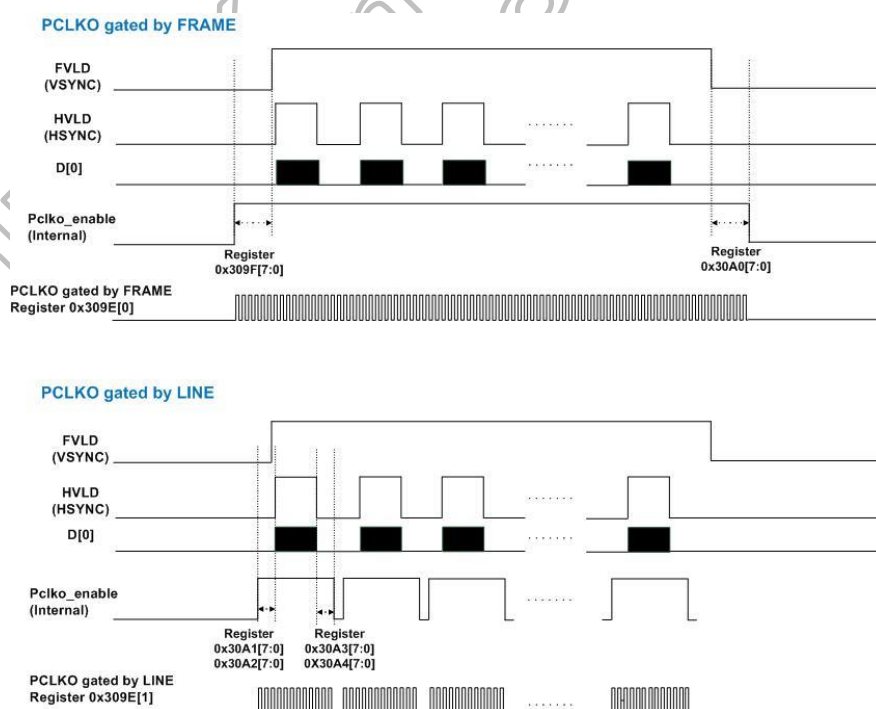
Figure 6.5: Gated serial data clock option
