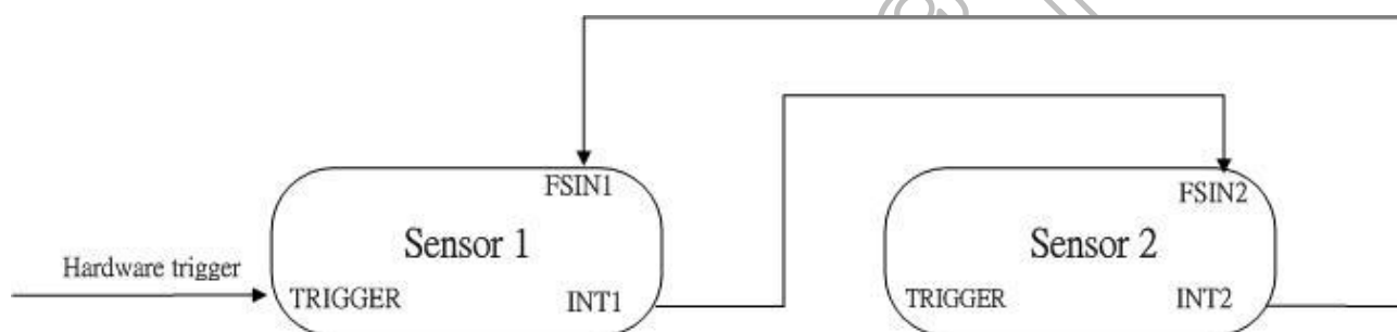
Figure 6.9: Block diagram for mode 1
