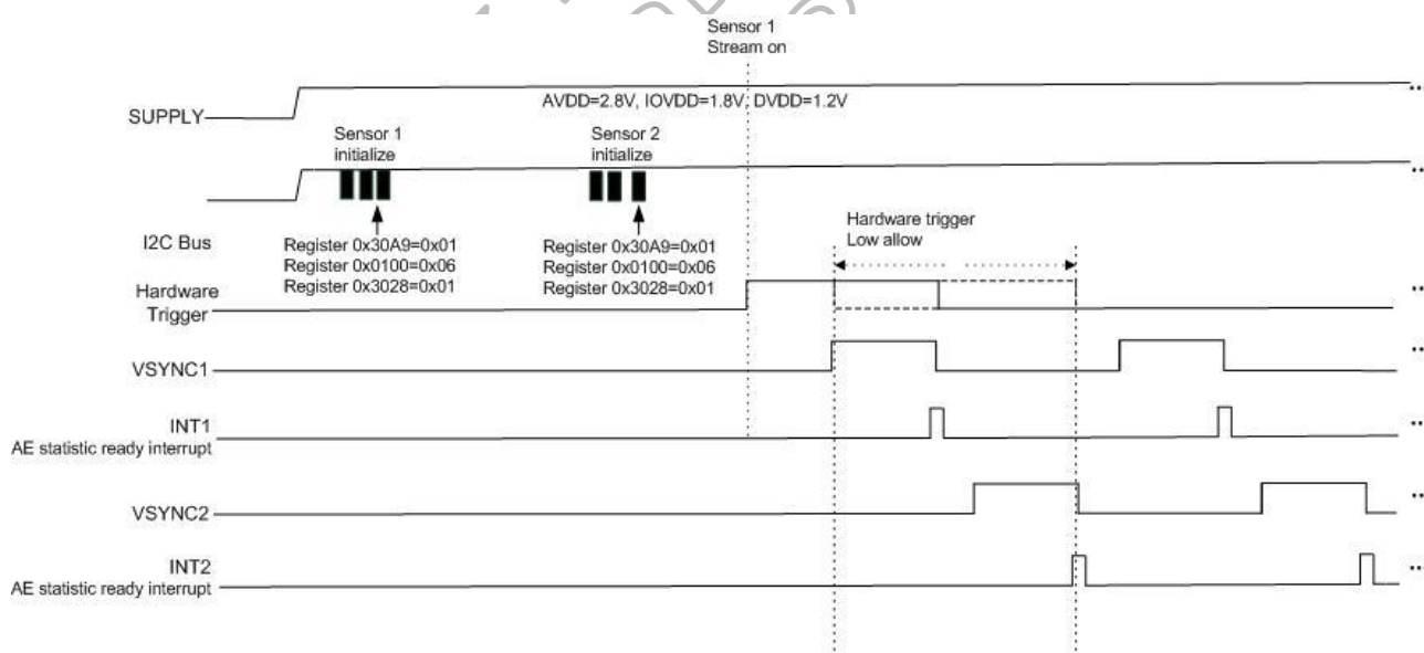
Figure 6.10: Operation scenario for mode 1
