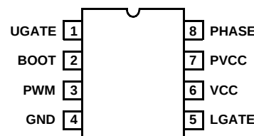
HIP6601CB/HIP6603CB (SOIC) TOP VIEW
