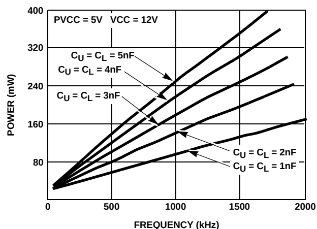
FIGURE 4. POWER DISSIPATION vs FREQUENCY (HIP6603)
