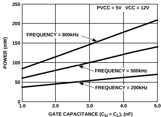
FIGURE 6. VARIABLE LOADING PROFILE (HIP6603)
