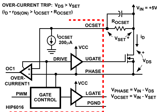
FIGURE 9. OVER-CURRENT DETECTION
