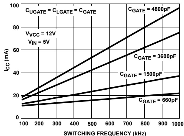
FIGURE 5. BIAS SUPPLY CURRENT vs FREQUENCY
