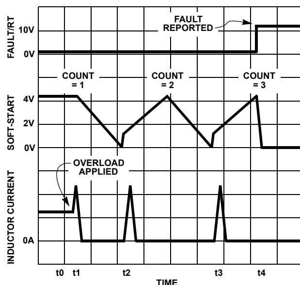
FIGURE 8. OVER-CURRENT OPERATION
