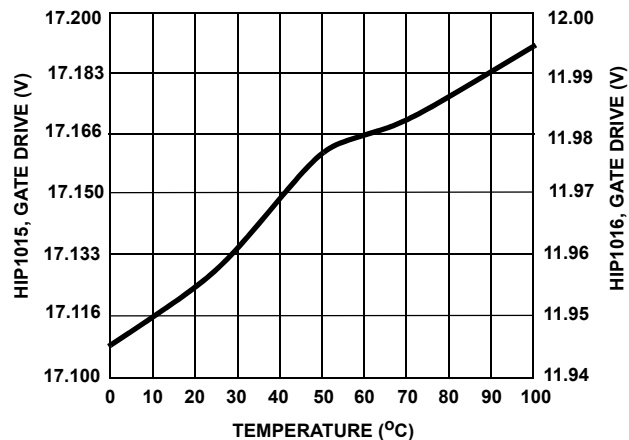
FIGURE 9. GATE DRIVE VOLTAGE, VDD = 12V
