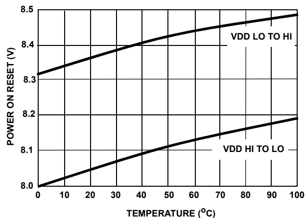
FIGURE 10. POWER ON RESET VOLTAGE THRESHOLD
