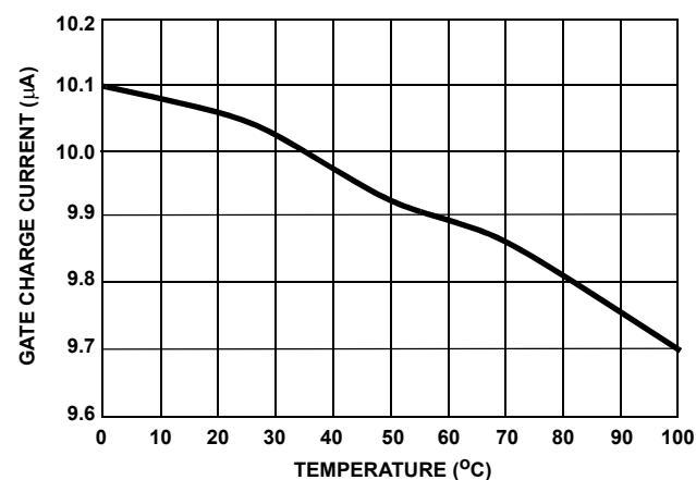
FIGURE 8. GATE CHARGE CURRENT
