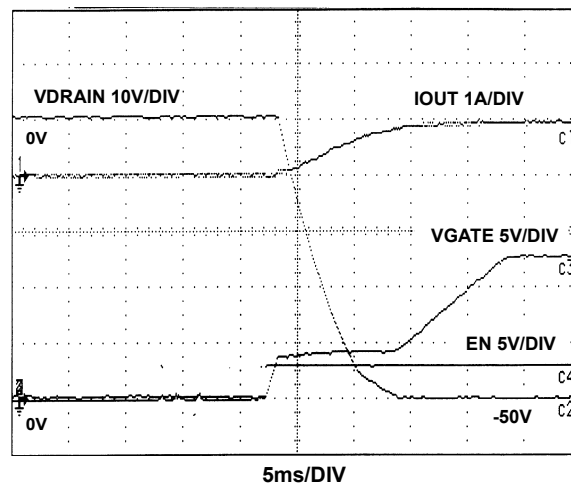
FIGURE 14. -50V LOW SIDE SWITCHING CGATE = 1000pF
