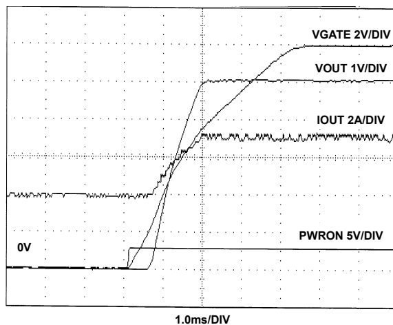
FIGURE 12. HIP1016 HIGH SIDE +5V TURN-ON
