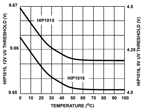
FIGURE 7. UV THRESHOLD
