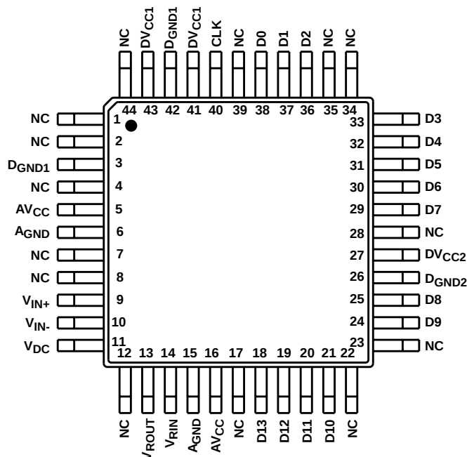
HI5905 (MQFP) (MO-108AA-2 ISSUE A) TOP VIEW
