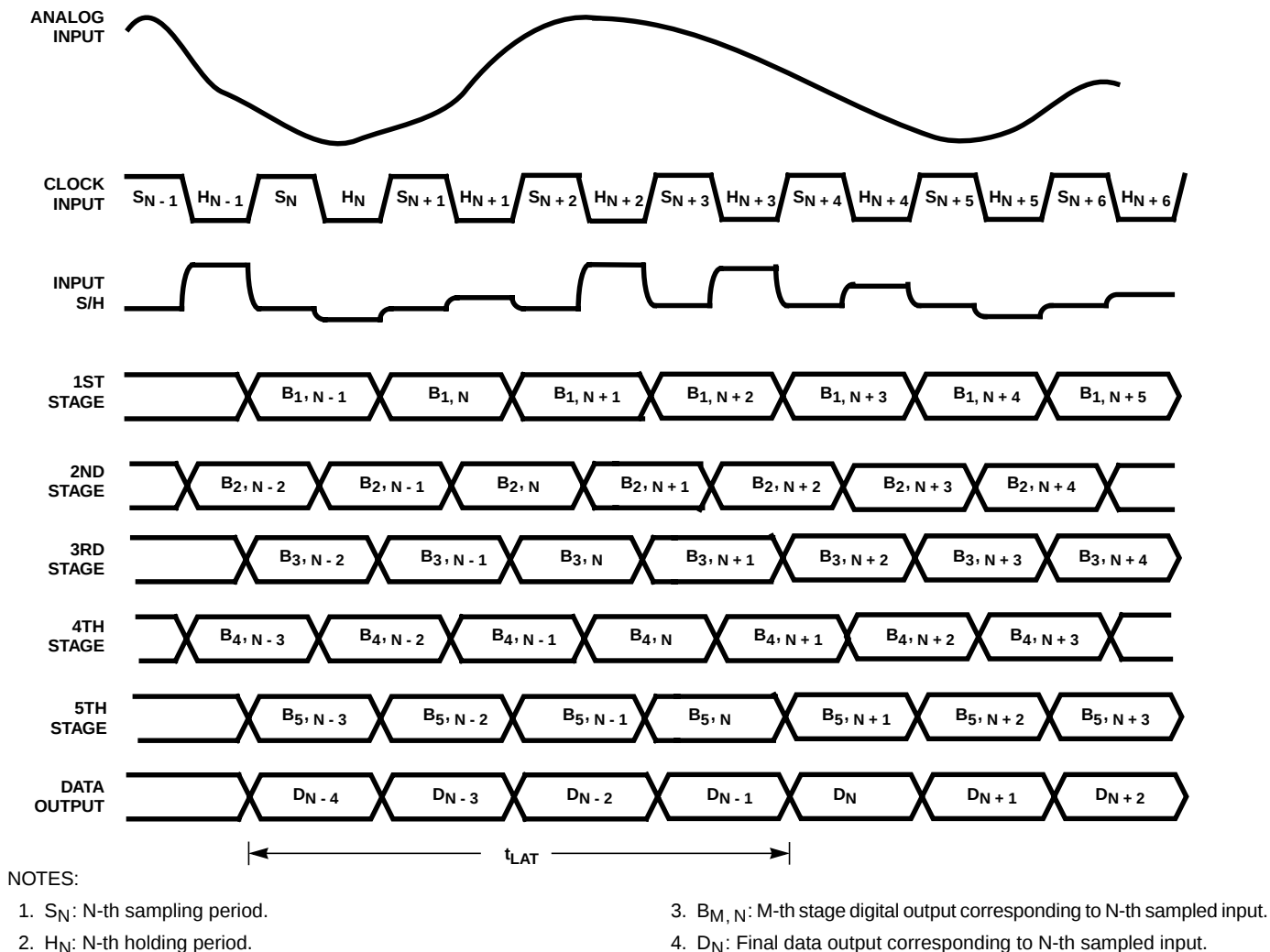
FIGURE 1. INTERNAL CIRCUIT TIMING
