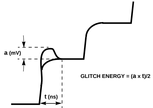
FIGURE 26. MEASURING GLITCH ENERGY
