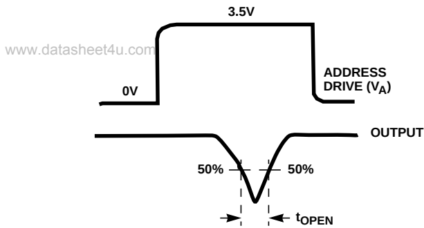
FIGURE 6B. MEASUREMENT POINTS
