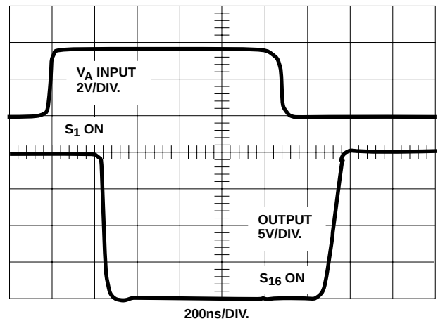
FIGURE 5D. WAVEFORMS
