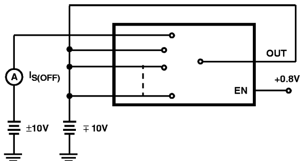
FIGURE 2C. I_{S(\text{OFF})} TEST CIRCUIT (NOTE 9)
