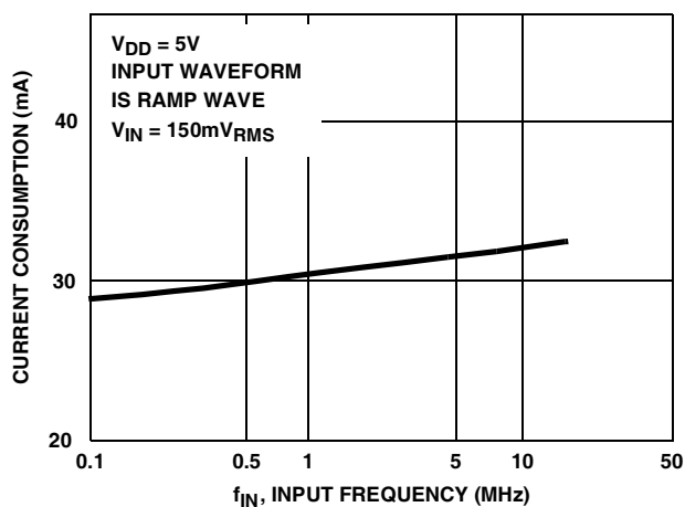
FIGURE 8. INPUT FREQUENCY vs CURRENT CONSUMPTION
