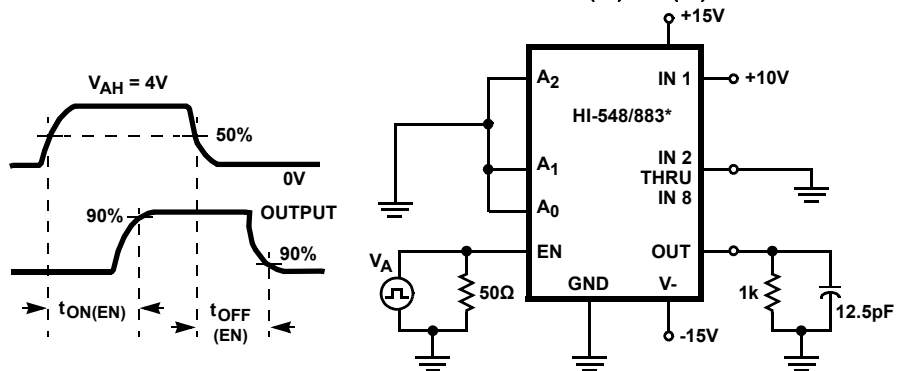
ENABLE DRIVE
