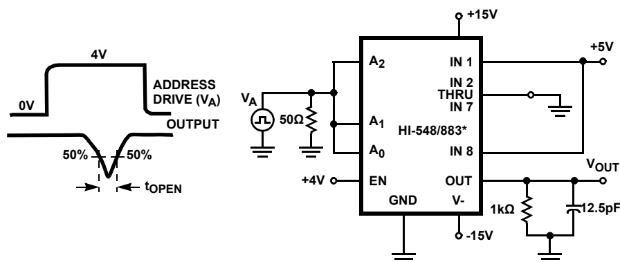
BREAK-BEFORE-MAKE DELAY ( t_{OPEN} )
