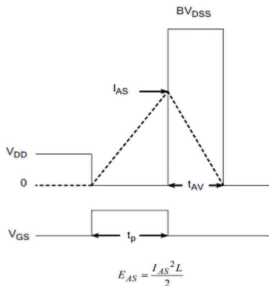
Figure21.Unclamped Inductive Switching
