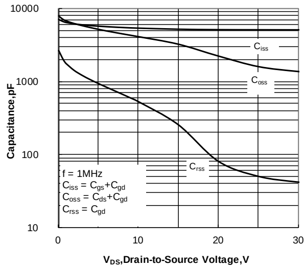
Figure 12. Capacitance Characteristics
