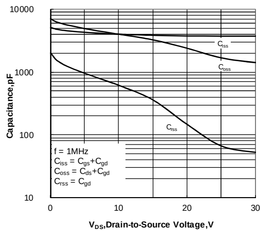
Figure 12. Capacitance Characteristics
