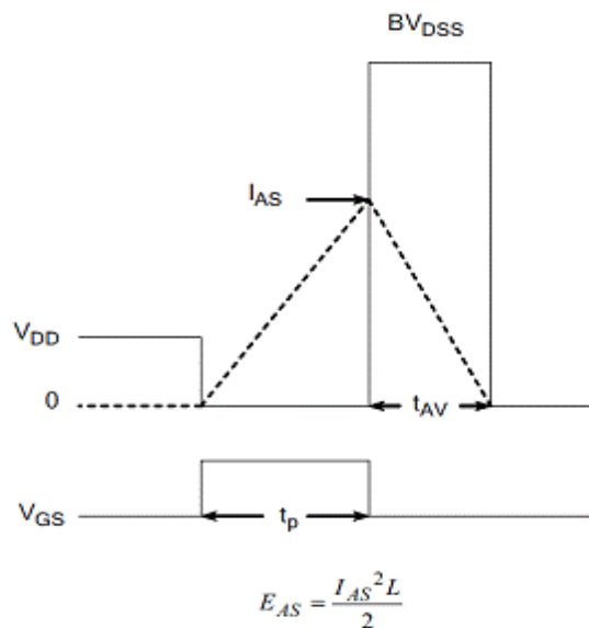
Figure21.Unclamped Inductive Switching
