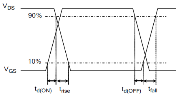
Figure 17. Resistive Switching
