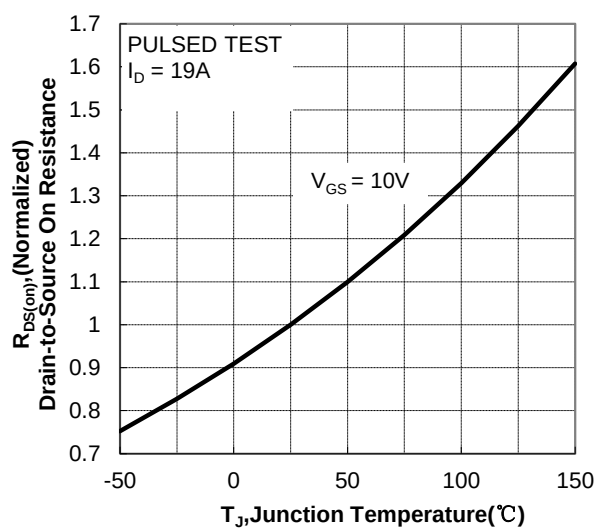
Figure 9. Normalized On Resistance vs Junction Temperature
