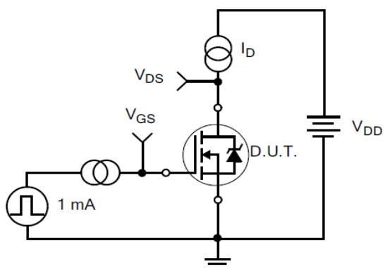
Figure 14. Gate Charge Test Circuit
