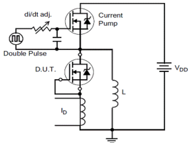
Figure 18. Diode Reverse Recovery Test Circuit
