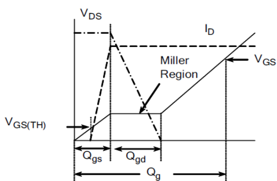
Figure 15. Gate Charge Wave forms
