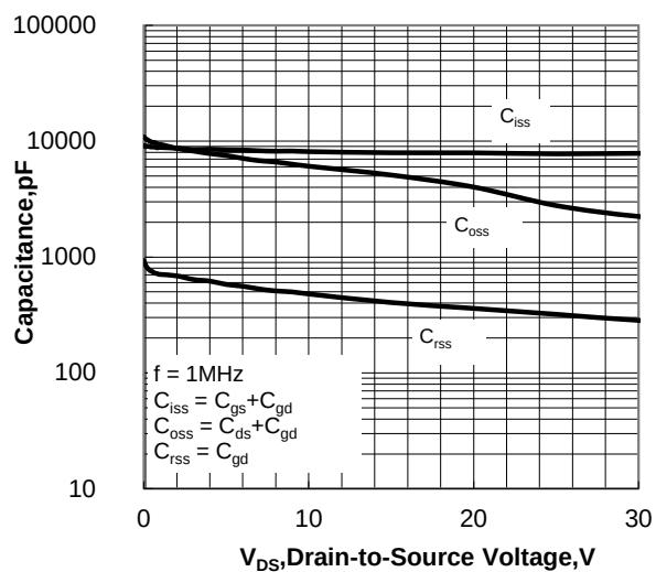
Figure 12. Capacitance Characteristics
