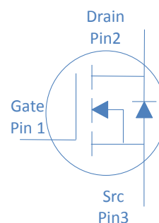
TO-220
