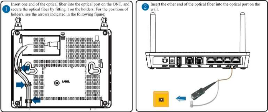
Figure 2-5 Optical ports on the HG8245H
