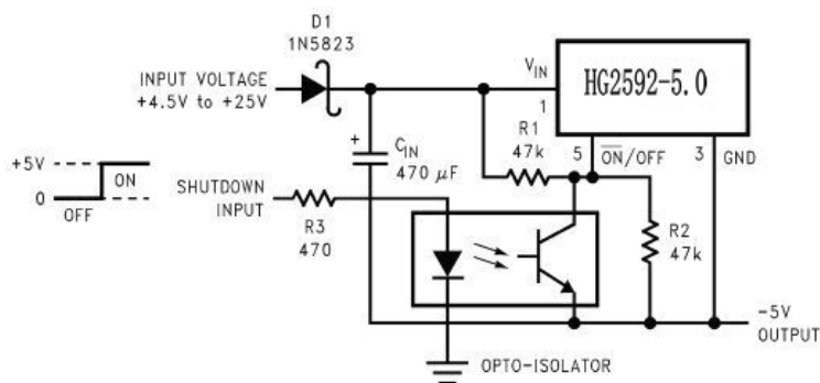
FIGURE 27. Inverting Regulator Ground Referenced Shutdown
