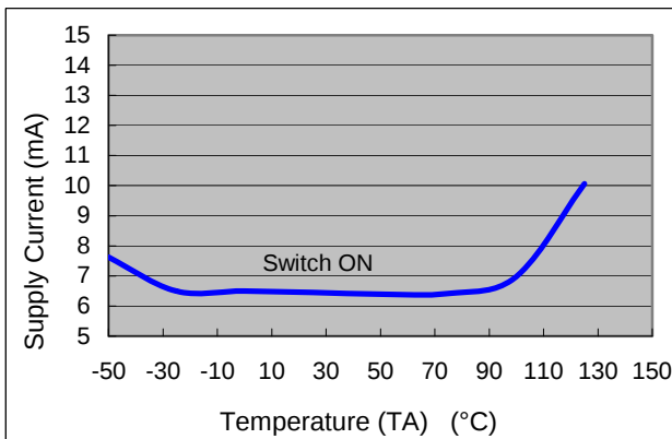
HG1509 Supply Current vs. Temperature ( V_{IN}=12V , No Load, V_{on/off}=0V (Switch ON), V_{on/off}=5V (Switch OFF))
