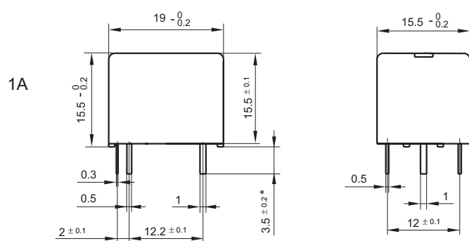
Outline Dimensions
