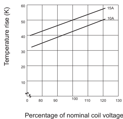
1. Coil temperature rise
