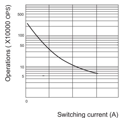
2. Electrical endurance curve
