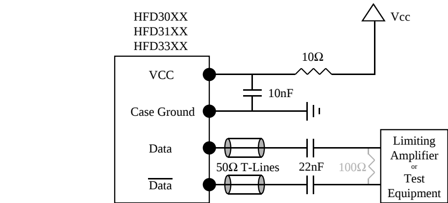
FIGURE 2: RECOMMENDED INTERFACE CIRCUIT FOR THE HFD3180-102
