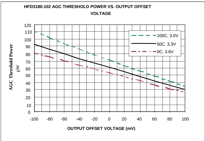
FIGURE 3: AGC THRESHOLD POWER VS. OUTPUT OFFSET VOLTAGE
