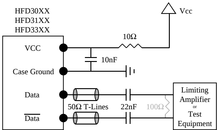
FIGURE 2: RECOMMENDED INTERFACE CIRCUIT FOR THE HFD3381-002
