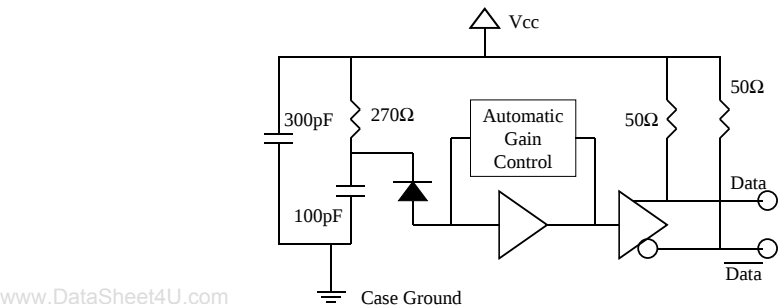
FIGURE 2: RECOMMENDED INTERFACE CIRCUIT FOR THE HFD3180-102
