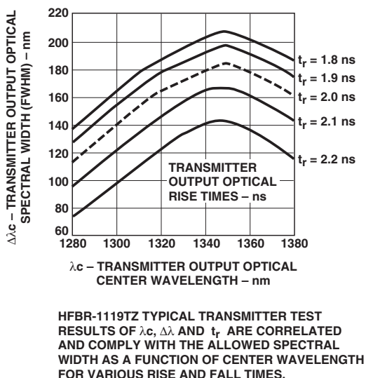
Figure 8. Typical transmitter output optical spectral width (FWHM) vs. transmitter output optical center wavelength and rise/fall times.
