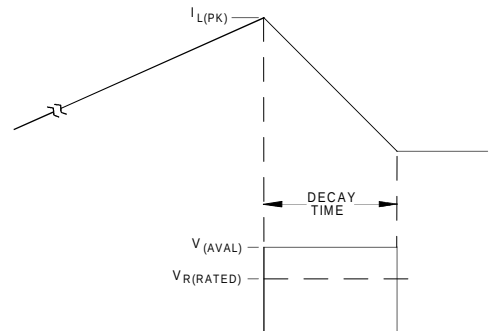
Fig. 11 - Avalanche Test Circuit and Waveforms
