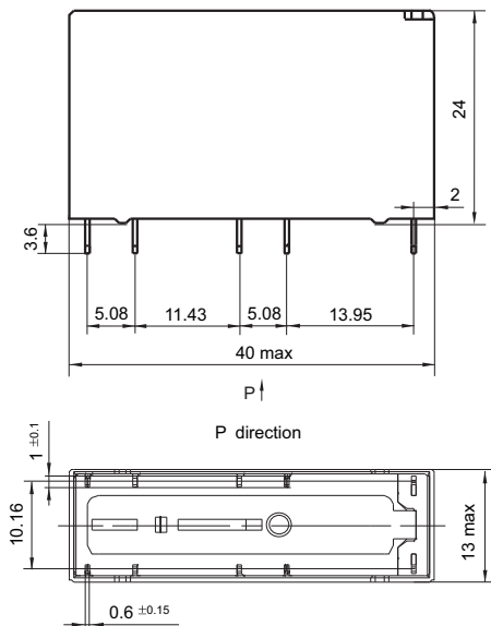
Outline Dimensions
