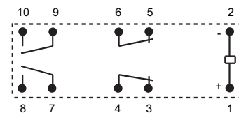
Wiring Diagram
