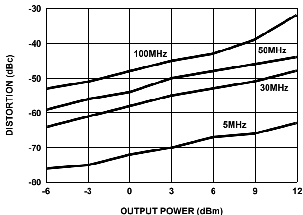
FIGURE 26. 2nd HARMONIC DISTORTION vs P_{\text{OUT}}
