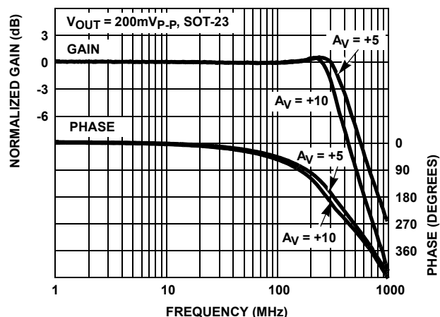
FIGURE 17. FREQUENCY RESPONSE
