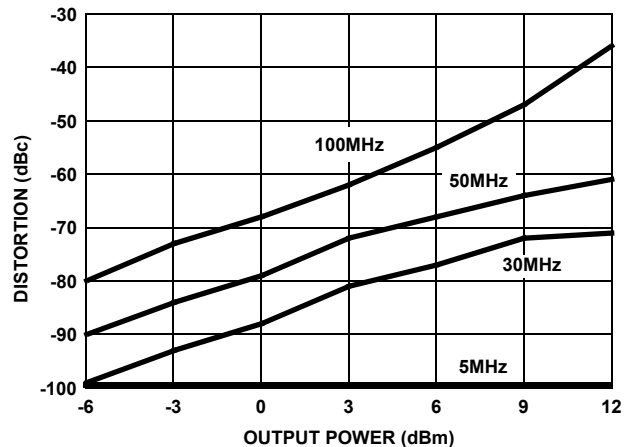
FIGURE 27. 3rd HARMONIC DISTORTION vs P_{\text{OUT}}
