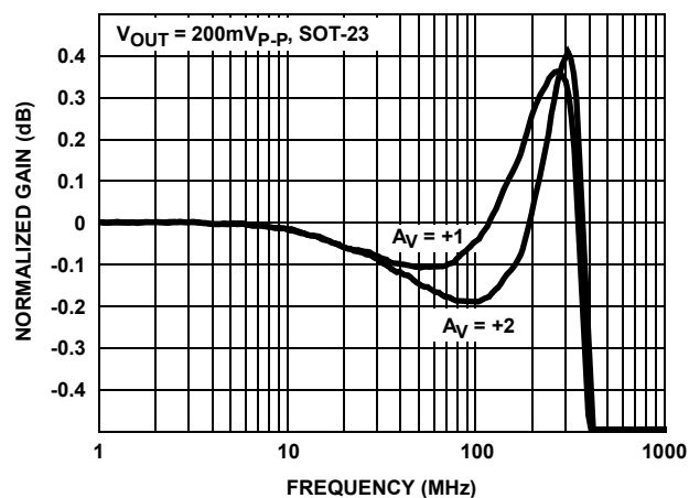
FIGURE 18. GAIN FLATNESS
