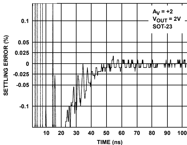
FIGURE 23. SETTLING RESPONSE
