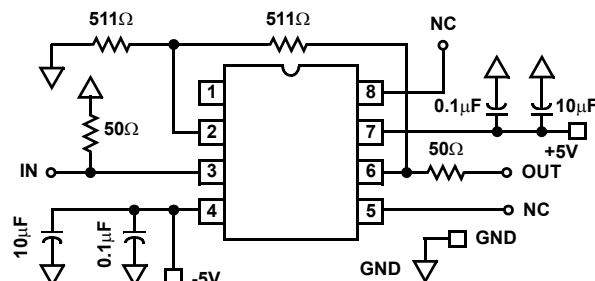
FIGURE 2. HFA11XXEVAL SCHEMATIC
