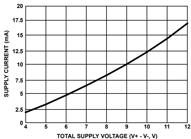
FIGURE 25. SUPPLY CURRENT vs SUPPLY VOLTAGE
