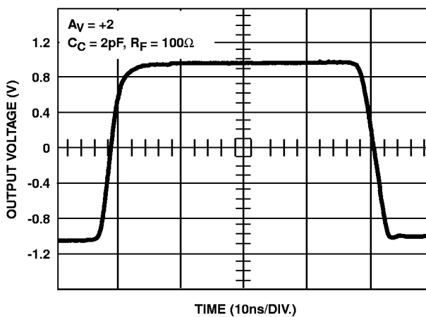
FIGURE 20. LARGE SIGNAL OUTPUT VOLTAGE
