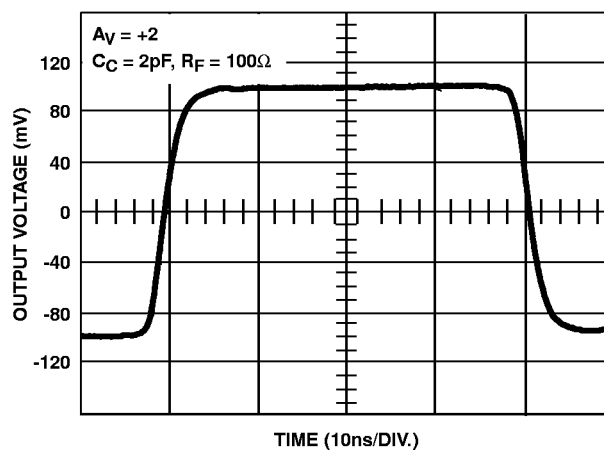
FIGURE 18. SMALL SIGNAL PULSE RESPONSE
