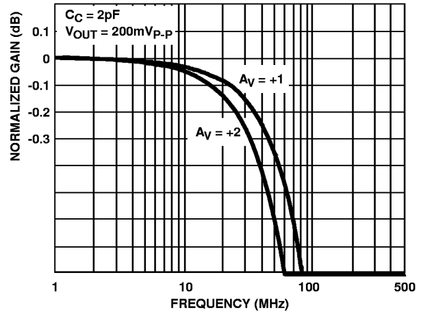
FIGURE 24. GAIN FLATNESS
