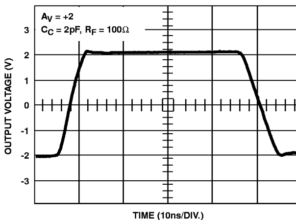
FIGURE 22. LARGE SIGNAL PULSE RESPONSE
