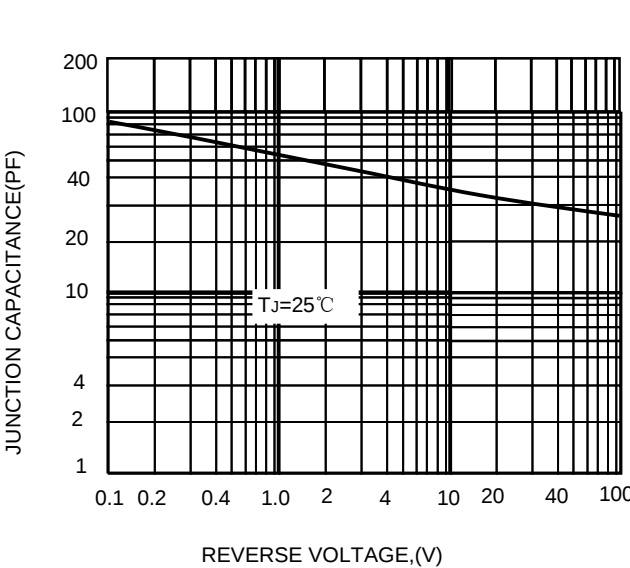
FIG.5-TYPICAL JUNCTION CAPACITANCE
