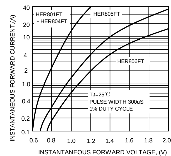
FIG.4-TYPICAL INSTANTAEIOUS FORWARD CHARACTERISTICS
