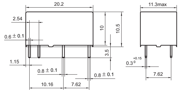
2 coils latching
