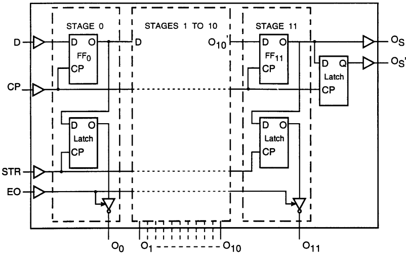
Fig.3 Logic diagram.
