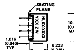
SIDE VIEW C, D, I
