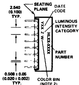
SIDE VIEW E, F, G, H
