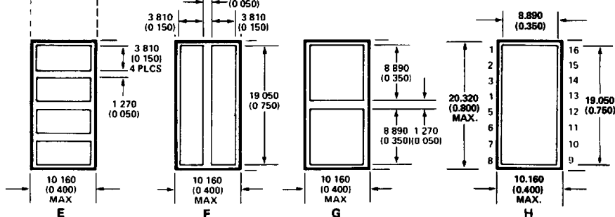
END VIEW C, D, E, F, G, H, I
