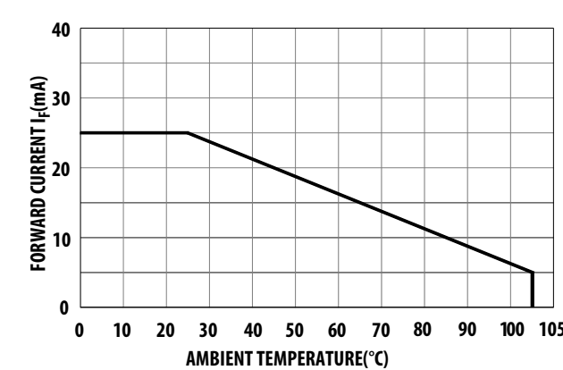
Figure 15: Allowable DC Current vs. Ambient Temperature
