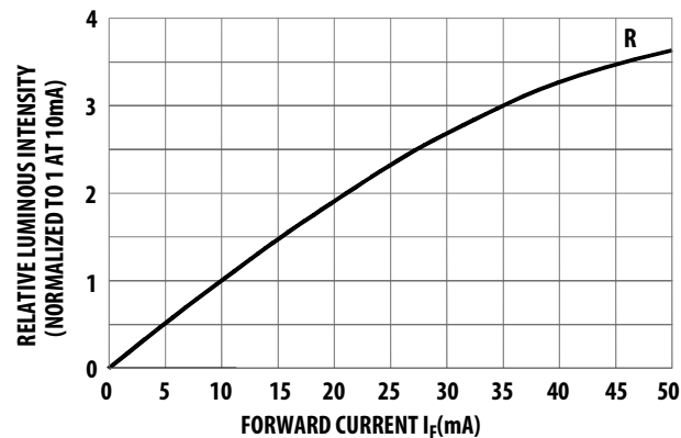
Figure 10: Relative Luminous Intensity vs. Forward Current
