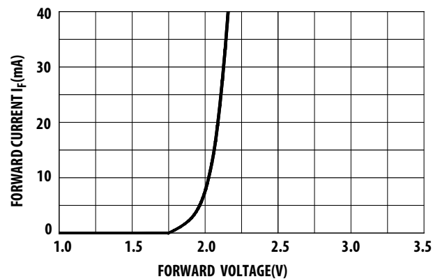
Figure 8: Forward Current vs. Forward Voltage
