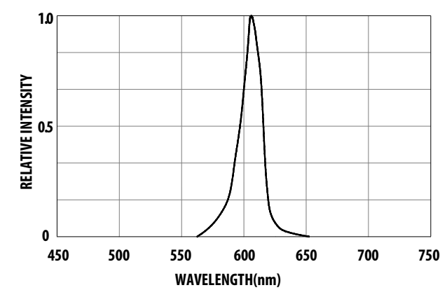
Figure 13: Relative Intensity vs. Wavelength
