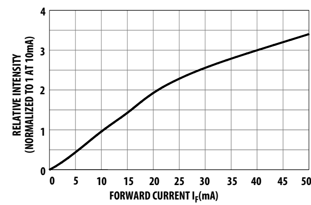
Figure 6: Relative Intensity vs. Forward Current
