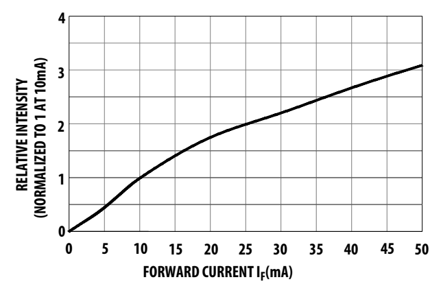
Figure 14: Relative Intensity vs. Forward Current
