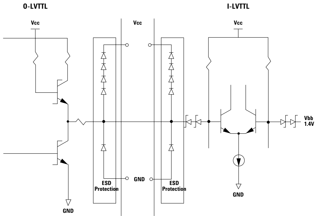
Figure 8. O_LVTTL and I_LVTTL Simplified Circuit Schematic.
