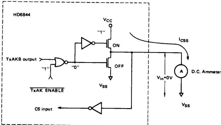
Figure 10 Source Current Measurement Circuit for CS/TxAKB Terminal
