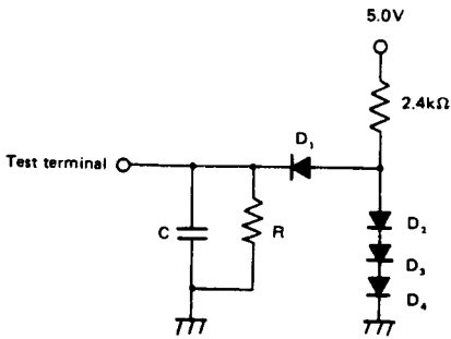
Figure 9 Load Circuit
