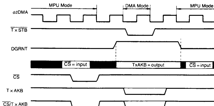
Figure 11A CS/TxAkB input/output Timing
