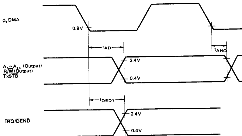
Figure 6 Timing of Address and \overline{\text{IRQ}}/\overline{\text{DEND}} Outputs
