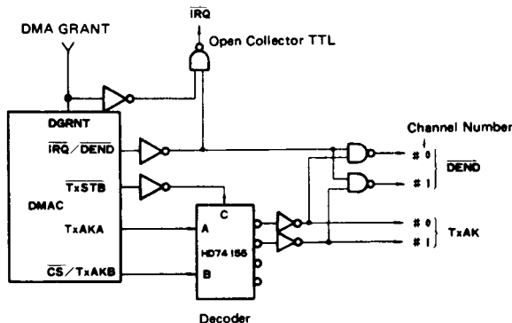
Figure 30 How to Use \overline{\text{IRQ}}/\text{DEND} Output Signal
