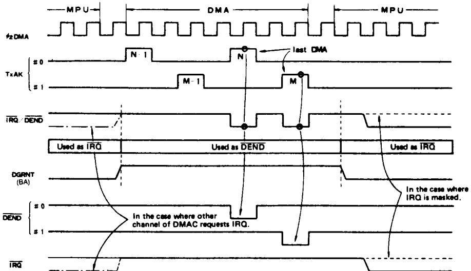
Figure 28 Logic of \overline{\text{IRQ}} Output
