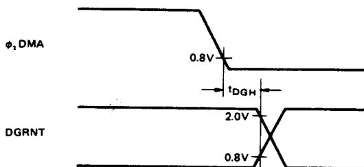
Figure 4 Timing of DGRNT Input
