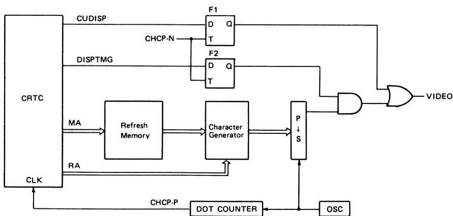
Figure 21 Display Control Unit (1)
