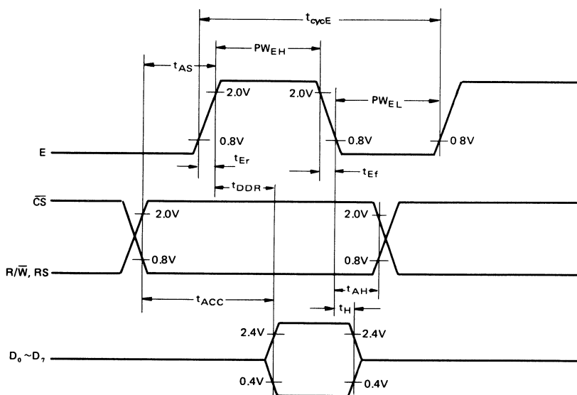
Figure 3 Read Sequence
