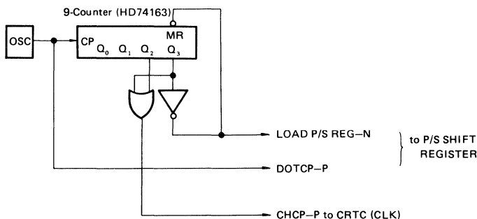
Figure 18 Example of Dot Counter
