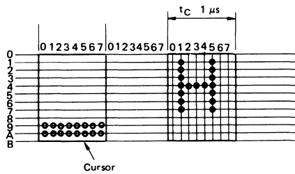
Figure 40 Non-interlace Display (Example)
