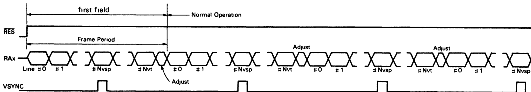
Figure 43 RES Release Sequence in The Non-interface Mode
