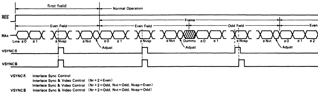
Figure 44 RES Release Sequence in The Interface Mode (1)
