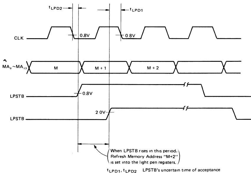
Figure 2 LPSTB Input Timing &amp; Refresh Memory Address that is set into the light pen registers.
