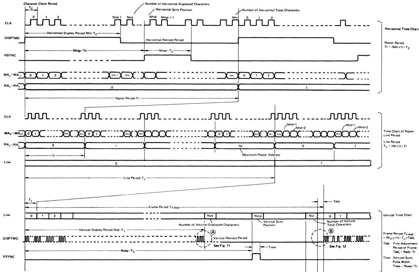
Figure 10 CRTC Time Chart
