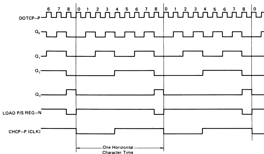
Figure 19 Time Chart of Dot Counter
