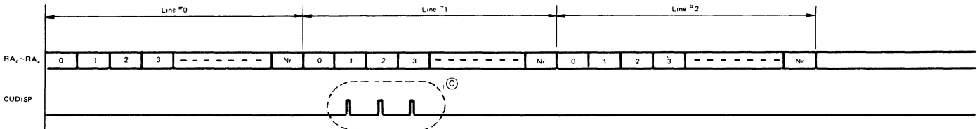
Figure 14 Relation between Line · Raster and CUDISP
