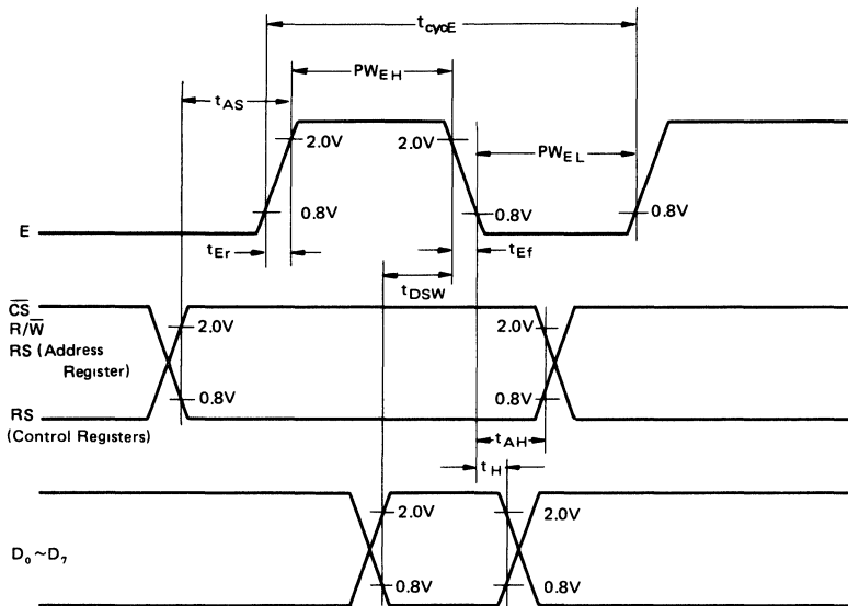
Figure 4 Write Sequence
