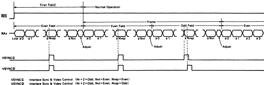
Figure 45 RES Release Sequence in The Interface Mode (2)
