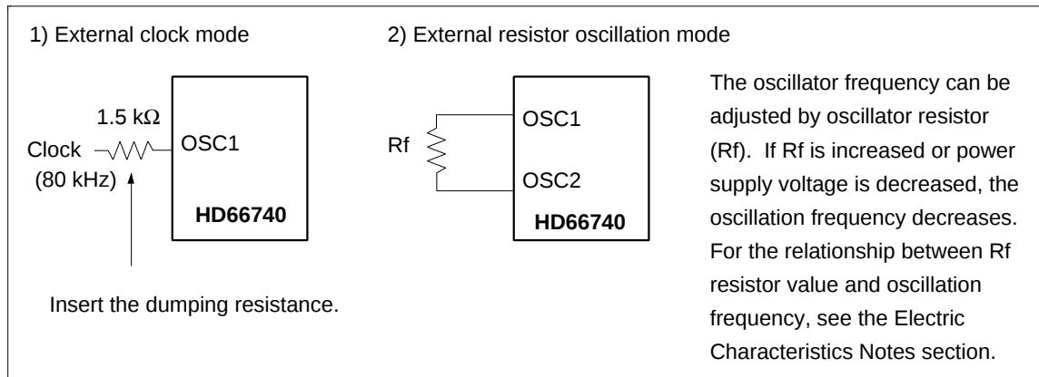
Figure 19 Oscillation Circuits
