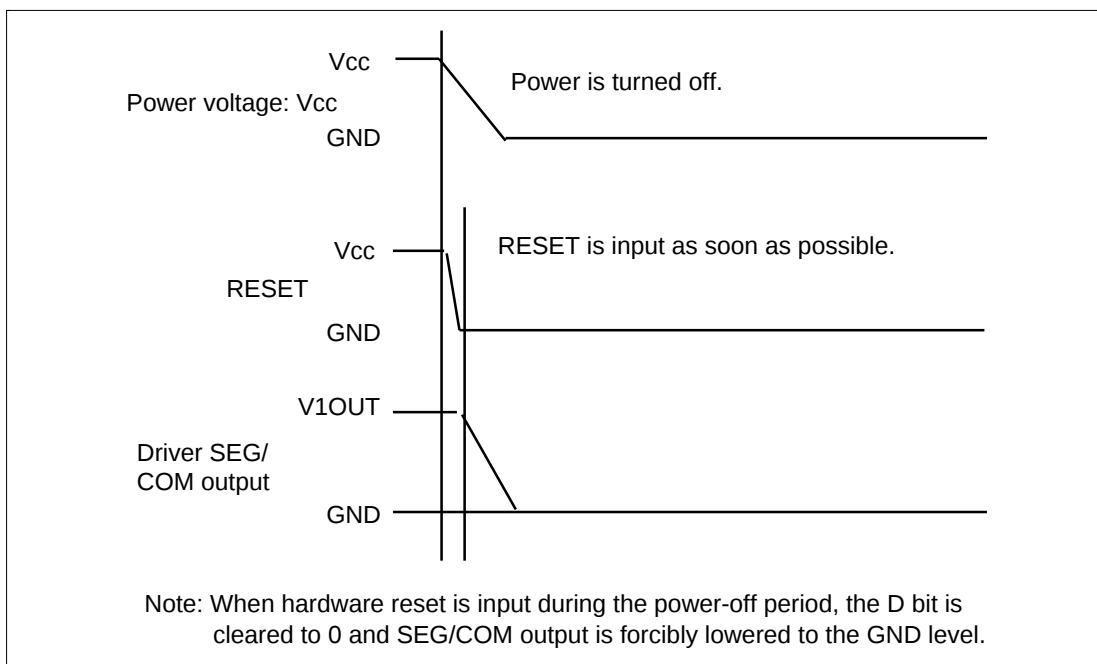
Figure 55 Power-off Timing
