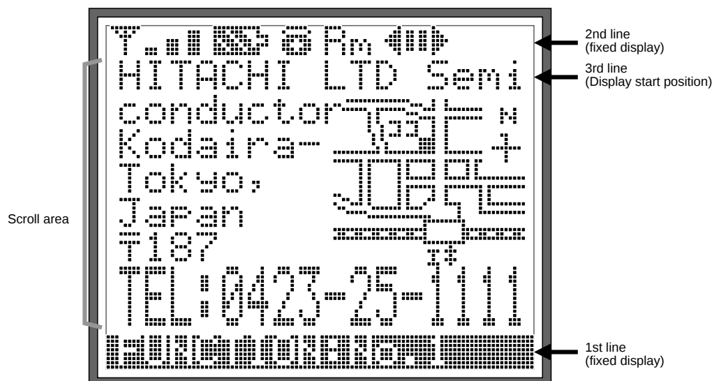
Figure 33 Example of Initial Screen in the Partial Smooth Scroll Mode
