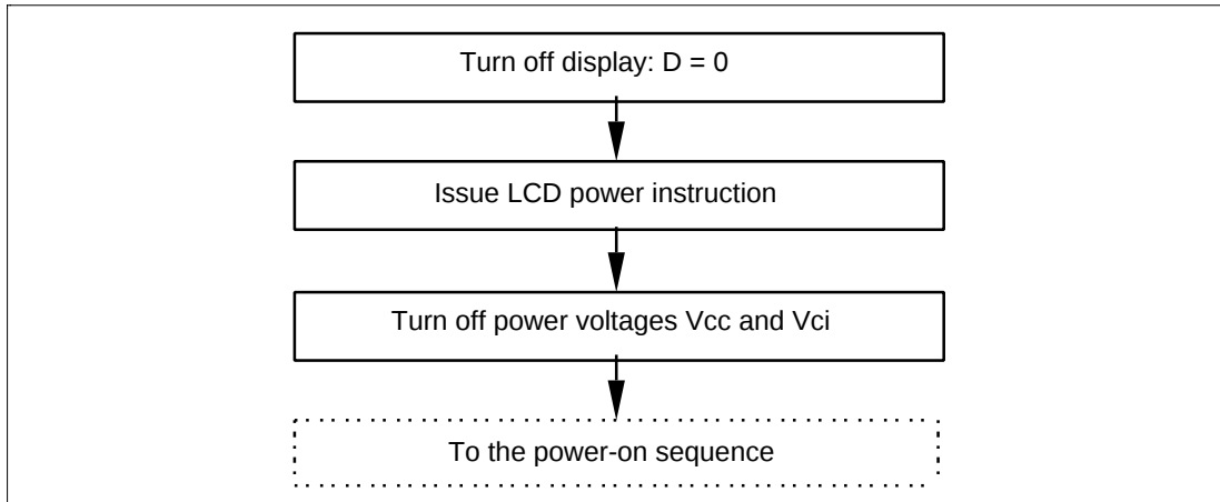
Figure 54 Power-off Sequence
