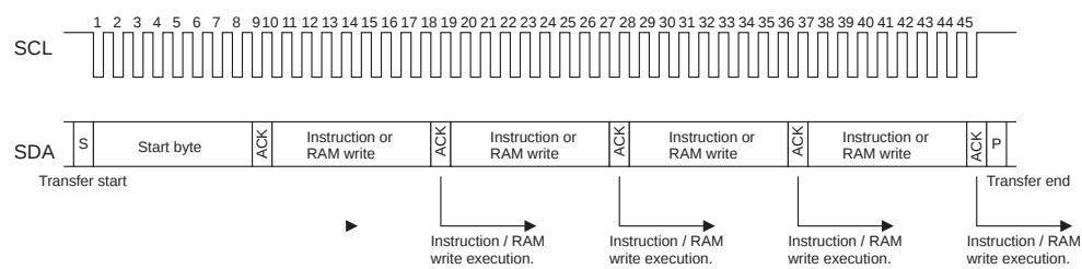
Figure 16-a I2C bus interface data-receive sequence
