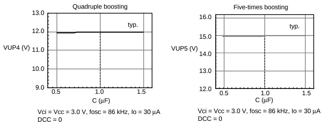
Figure 45 Booster (cont)
