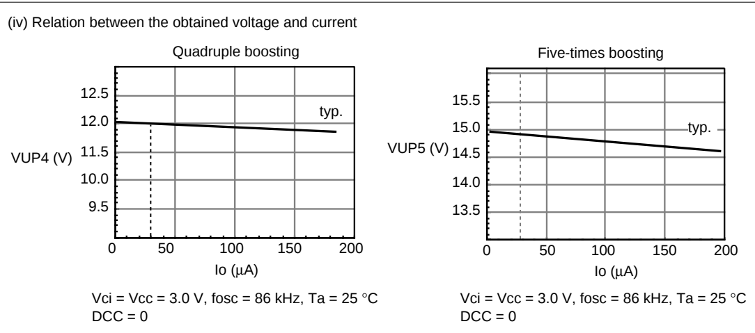
Figure 45 Booster (cont)
