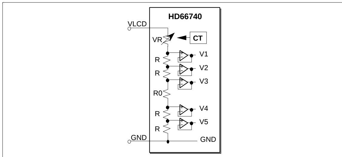
Figure 27 Contrast Adjuster
