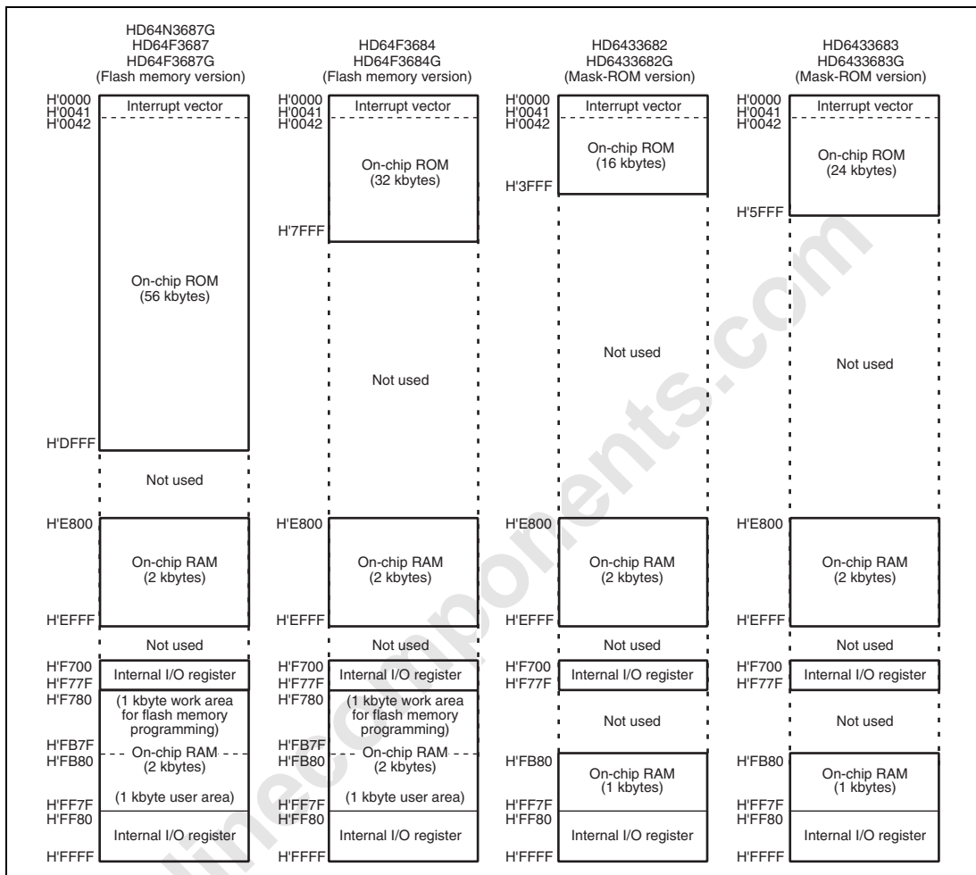
Figure 2.1 Memory Map (1)
