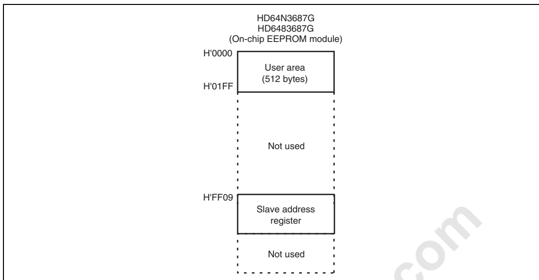
Figure 2.1 Memory Map (3)
