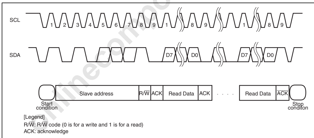
Figure 19.7 Sequential Read Operation (when current address read is used)
