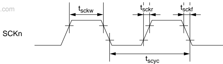
Figure 22.32 Input Clock Timing
