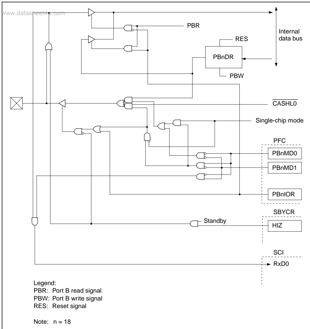
Figure C.8 PB18/CASHL0/RxD0 Block Diagram
