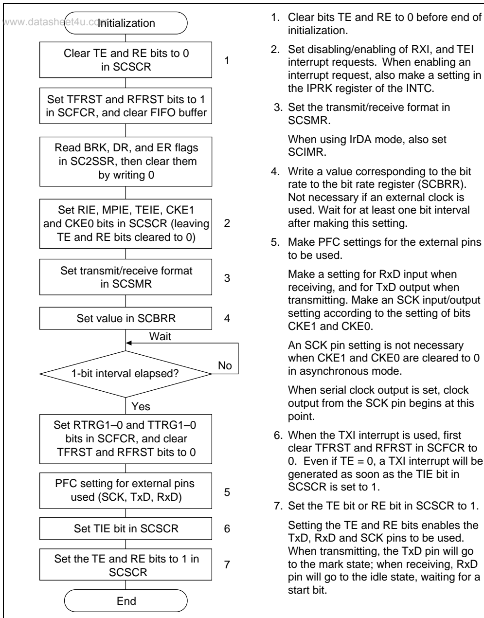
Figure 14.4 Sample SCI Initialization Flowchart
