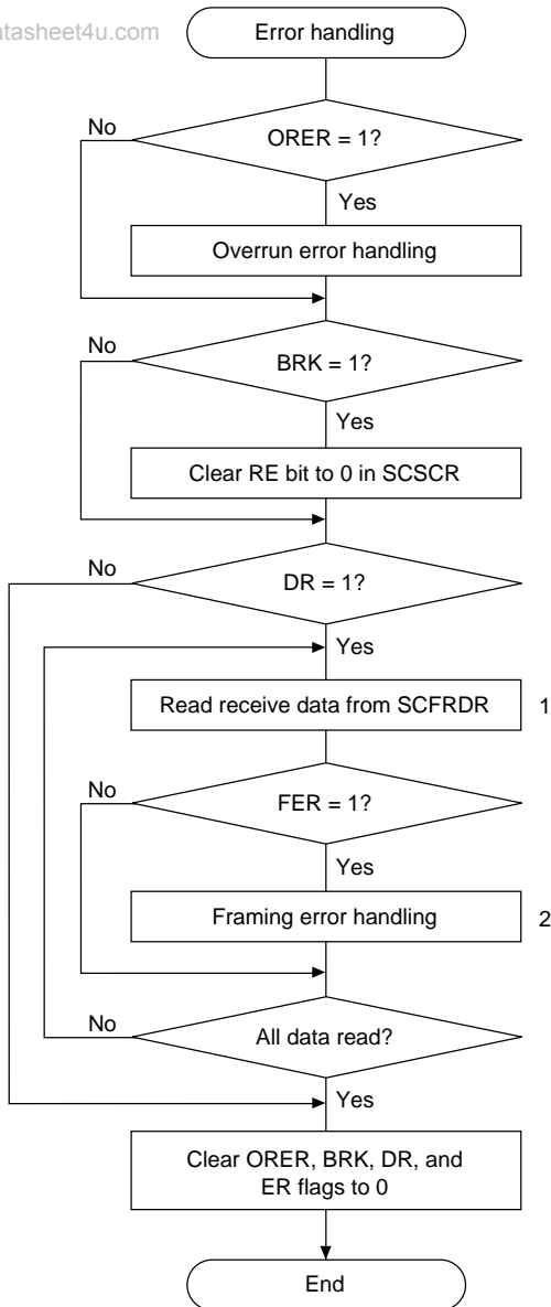
Figure 14.14 Sample Multiprocessor Serial Reception Flowchart (2)
