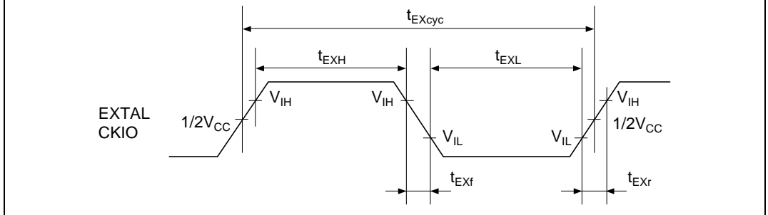
Figure 22.3 EXTAL Clock Input Timing
