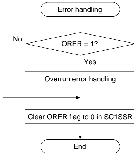
Figure 14.21 Sample Serial Reception Flowchart (2)
