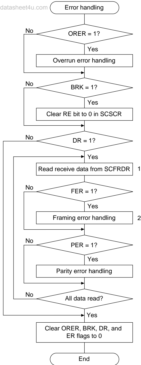
Figure 14.8 Sample Serial Reception Flowchart (2)
