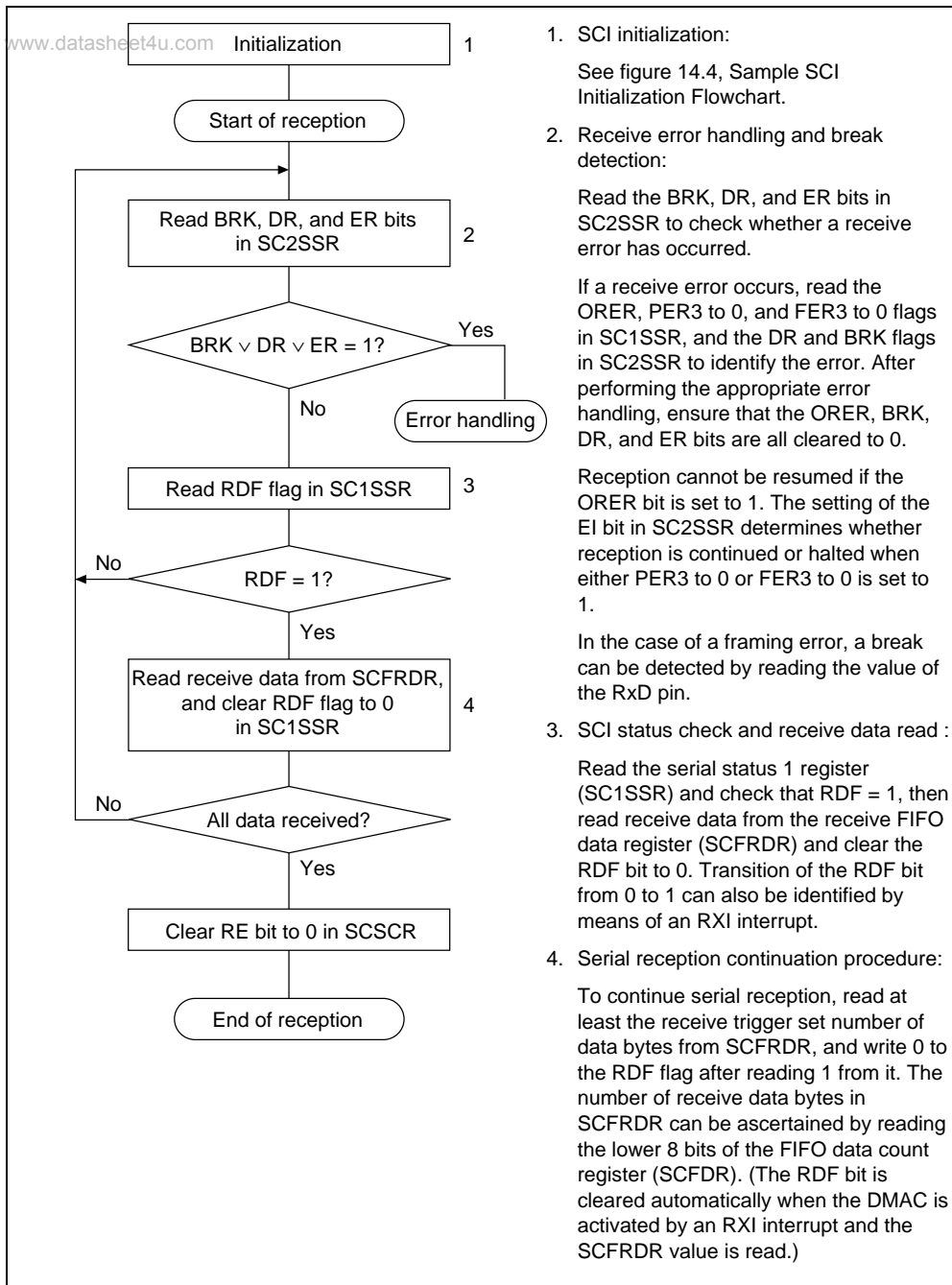
Figure 14.7 Sample Serial Reception Flowchart (1)
