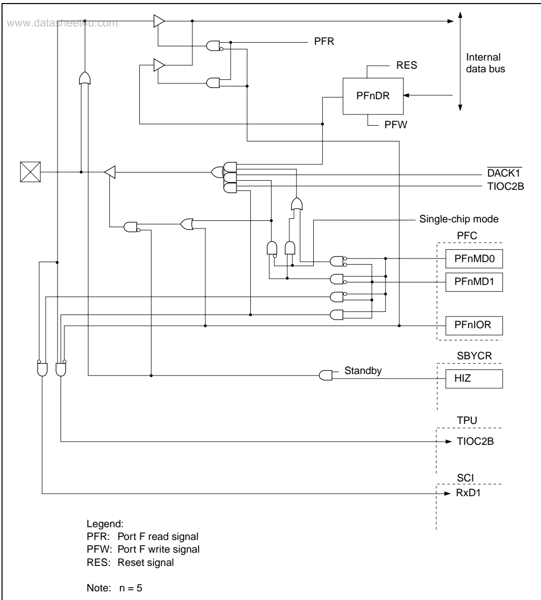
Figure C.41 PF5/DACK1/RxD1/TIOC2B Block Diagram
