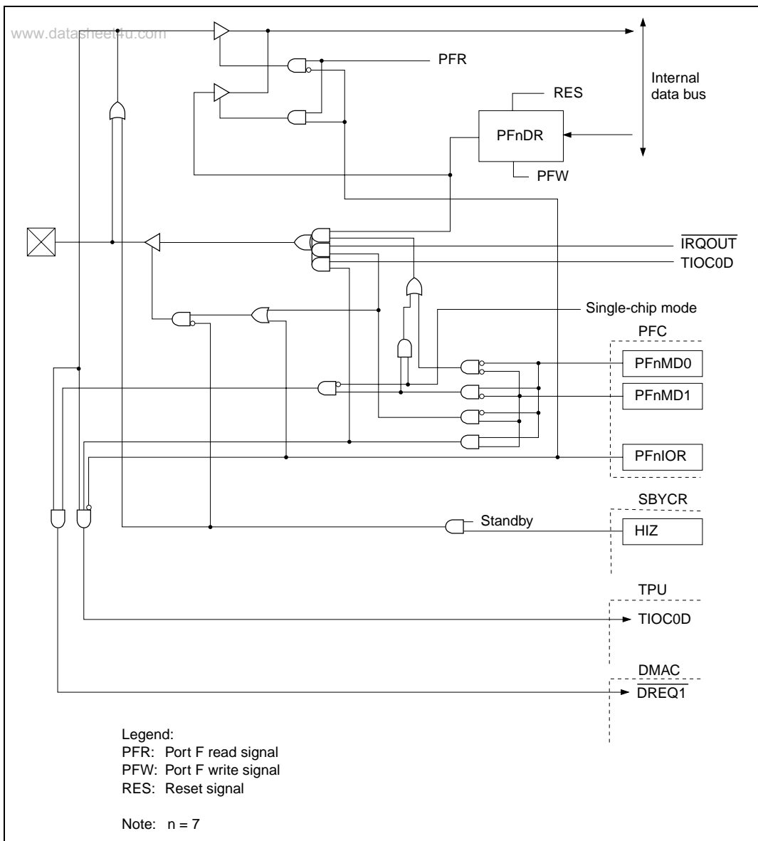
Figure C.43 PF7/ DREQ1 / IRQOUT / TIOC0D Block Diagram
