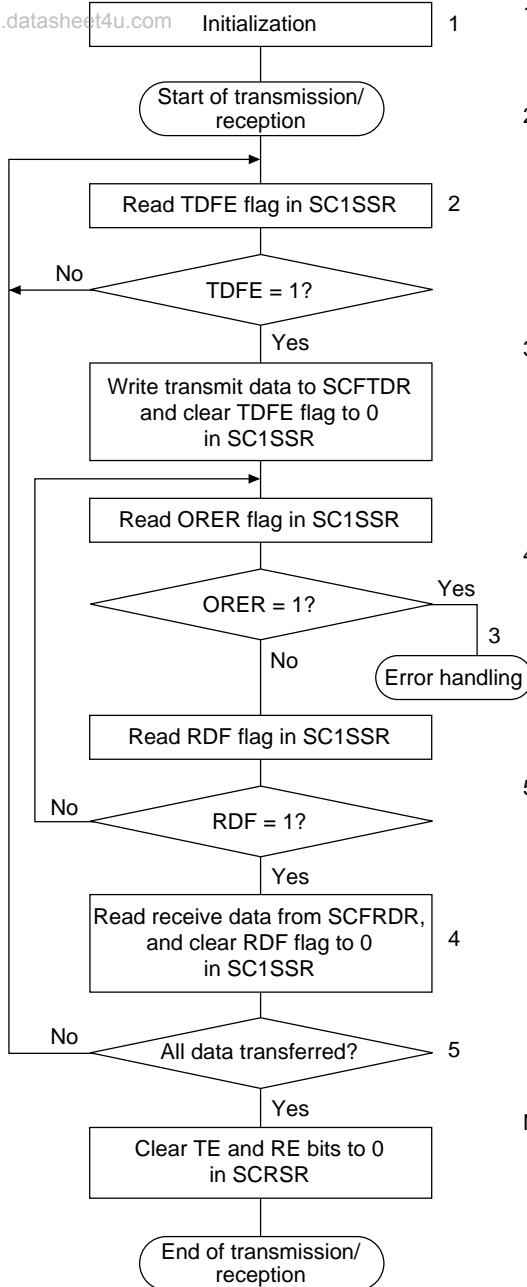
Figure 14.23 Sample Flowchart for Serial Transmission and Reception
