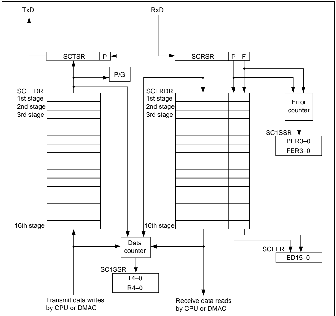
Figure 14.24 Transmit/Receive FIFO Configuration
