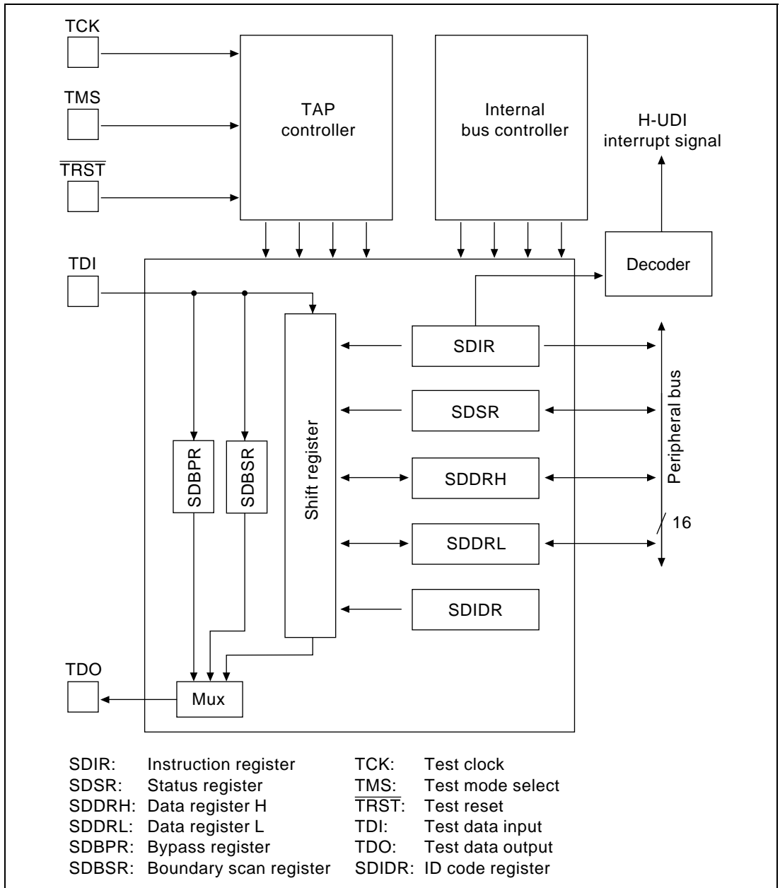
Figure 19.1 H-UDI Block Diagram
