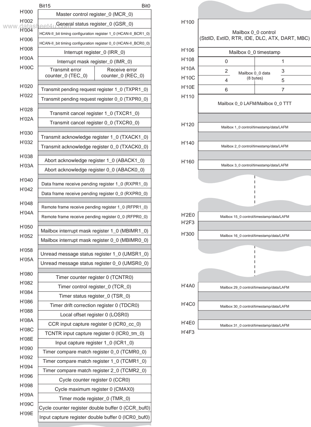
Figure 16.2 (1) HCAN-II Memory Map for Channel 0 (HCAN0)
