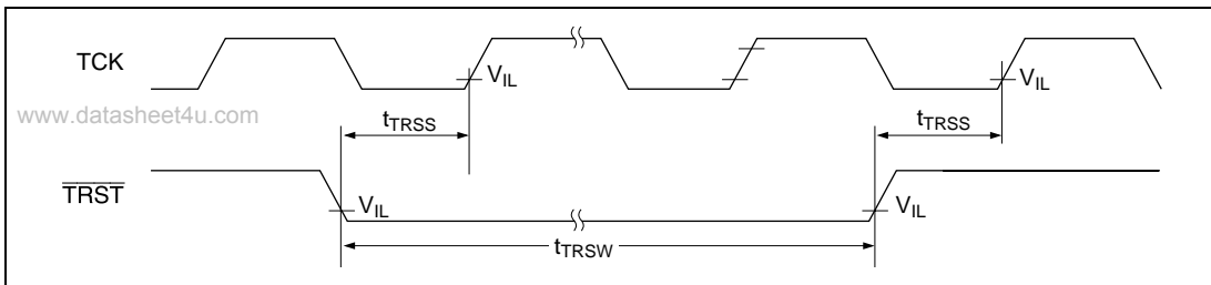
Figure 27.22 H-UDI \overline{TRST} Timing
