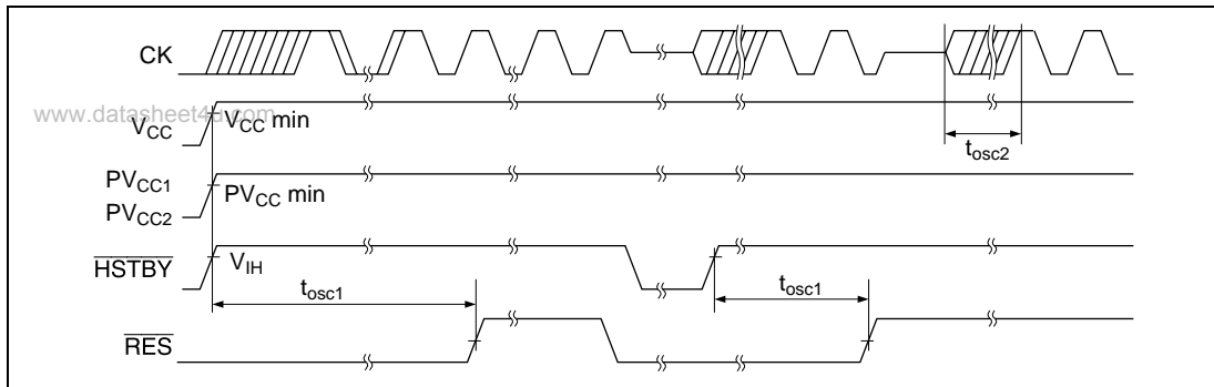
Figure 27.4 Oscillation Settling Time
