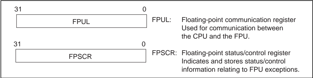
Figure 2.5 Floating-Point System Registers
