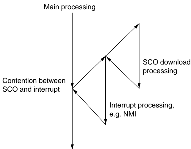
Figure 23.22 Contention between Interrupts (e.g. NMI)
