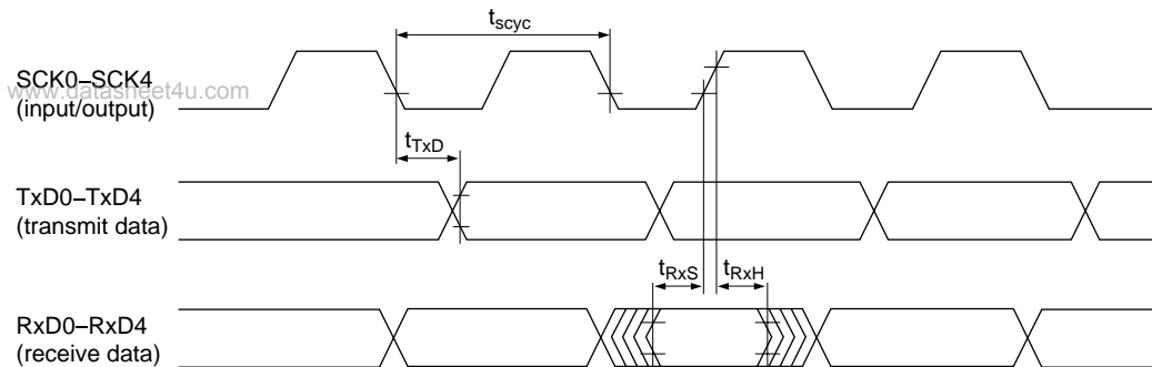
SCI input/output timing (synchronous mode)
