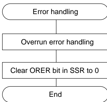
Figure 15.21 Sample Flowchart for Serial Receiving (2)
