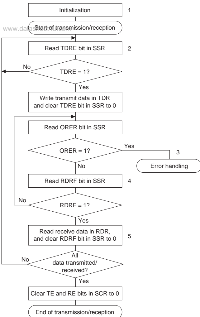
Figure 15.23 Sample Flowchart for Serial Transmission and Reception
