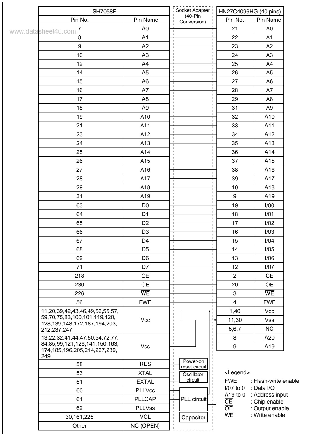
Figure 23.25 Pin Arrangement of Socket Adapter
