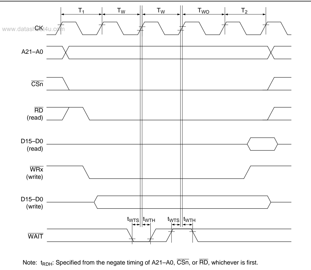
Figure 27.11 Basic Cycle (Two Software Waits + Waits by \overline{WAIT} Signal)
