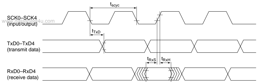
SCI input/output timing (clock synchronous mode)
