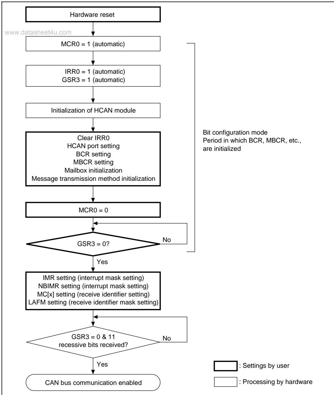
Figure 16.5 Hardware Reset Flowchart
