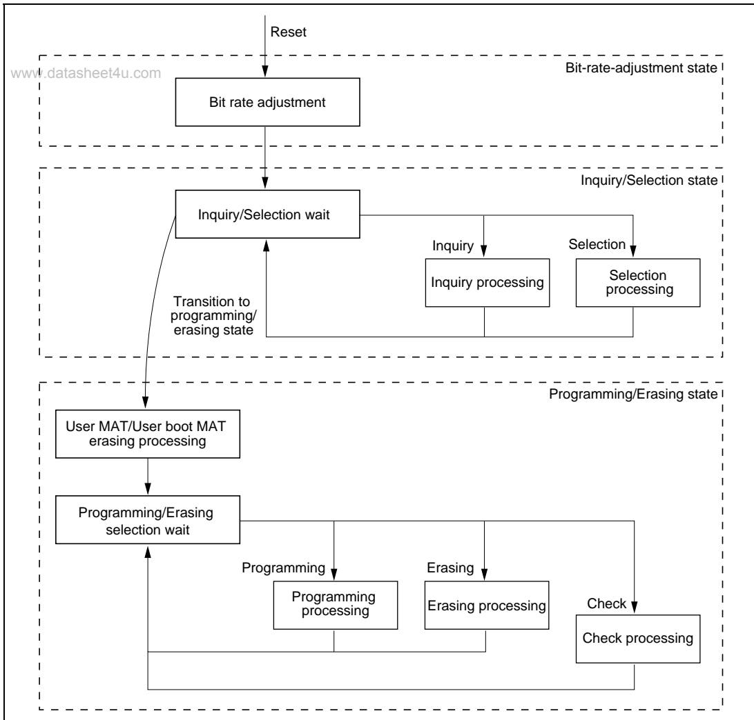
Figure 22.26 Boot Program Processing Flow
