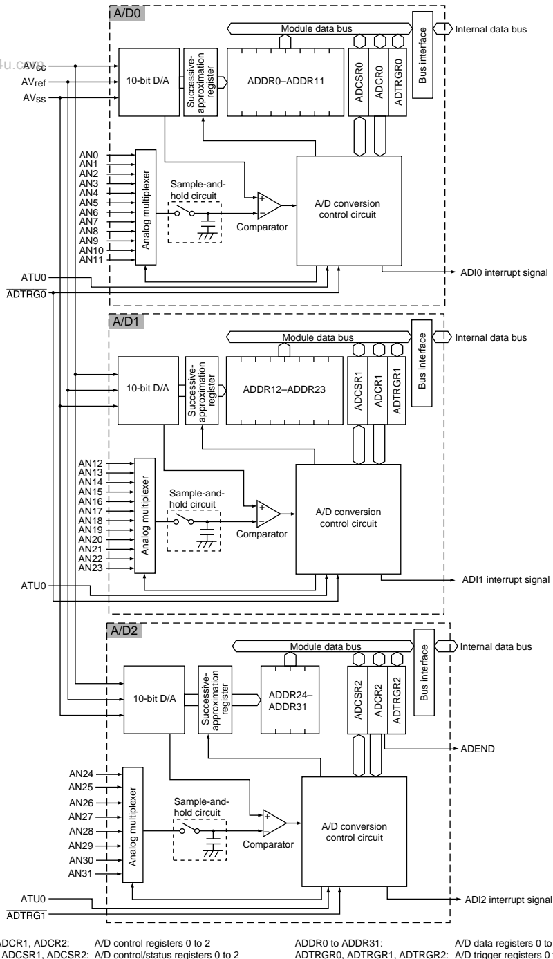
Figure 17.1 A/D Converter Block Diagram
