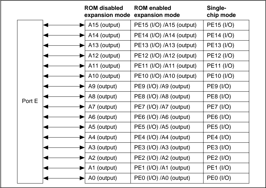
Figure 21.5 Port E
