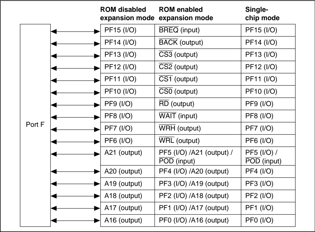
Figure 21.6 Port F
