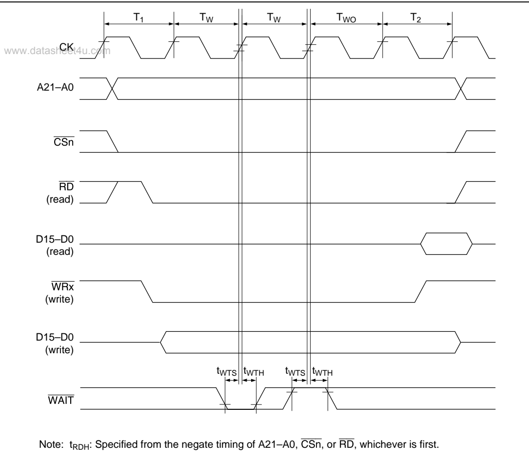
Figure 26.11 Basic Cycle (Two Software Waits + Waits by \overline{\text{WAIT}} Signal)
