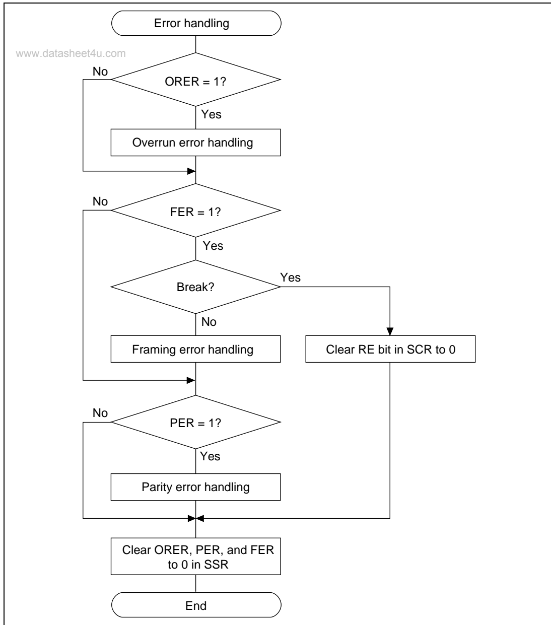
Figure 15.8 Sample Flowchart for Receiving Serial Data (2)
