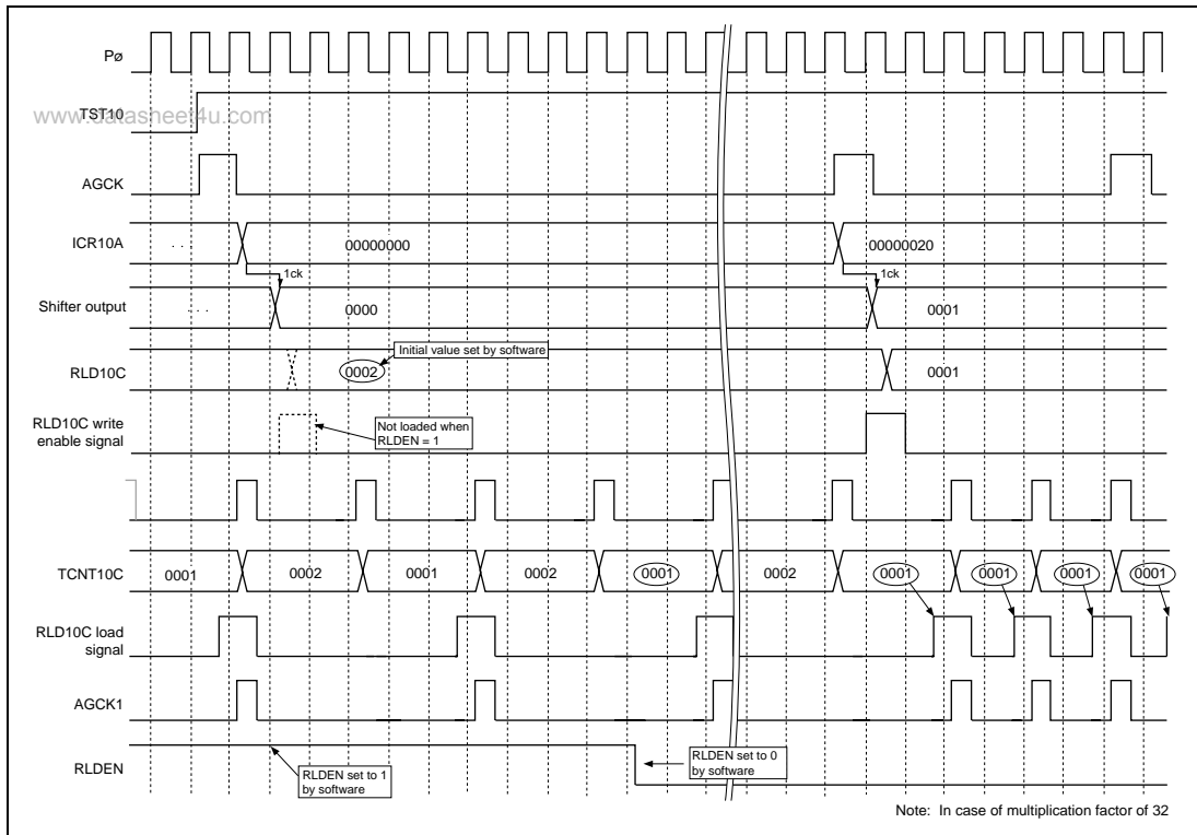
Figure 11.30 TCNT10C Operation
