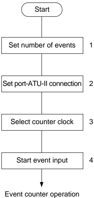
Figure 11.61 Sample Setup Procedure for Event Counter Operation
