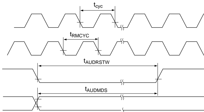
Figure 26.24 AUD Reset Timing
