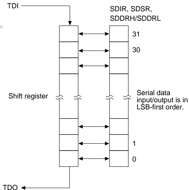
Figure 18.5 Serial Data Input/Output
