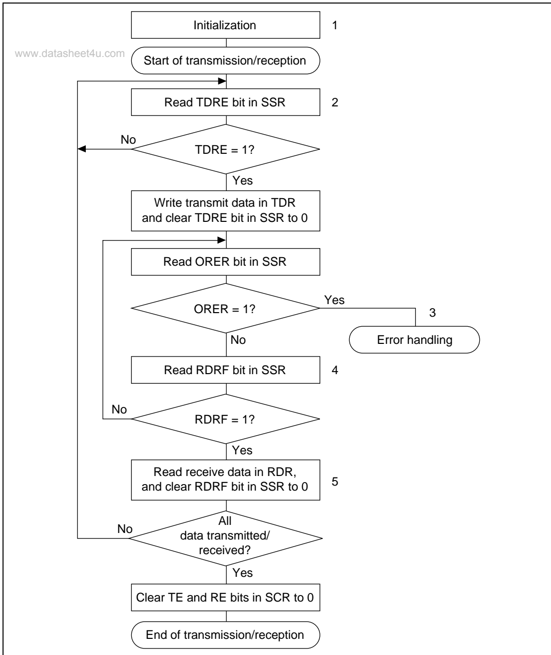
Figure 15.24 Sample Flowchart for Serial Transmission and Reception
