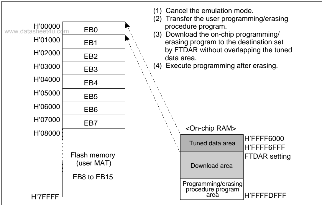
Figure 22.19 Programming of Tuned Data
