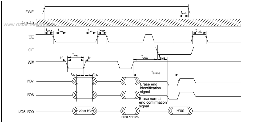
Figure 22.37 Timing in Auto-Erase Mode
