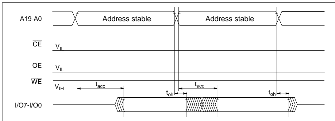
Figure 22.34 \overline{CE}/\overline{OE} Enable State Read
