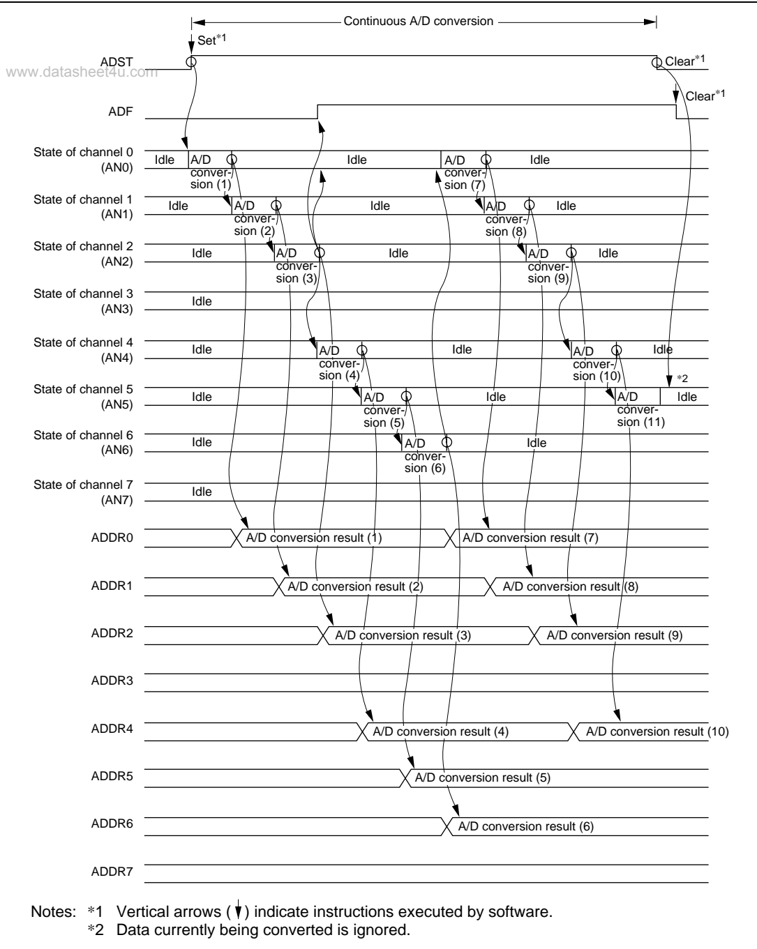
Figure 17.5 Example of A/D Converter Operation (Scan Mode (Continuous Scan), Channels AN0 to AN2 and AN4 to AN6 Selected)
