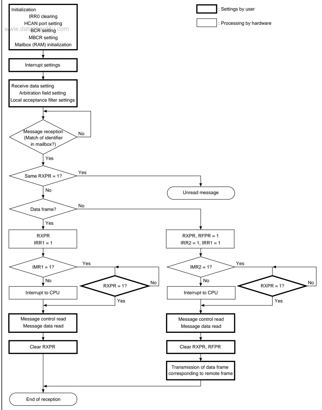
Figure 16.11 Reception Flowchart
