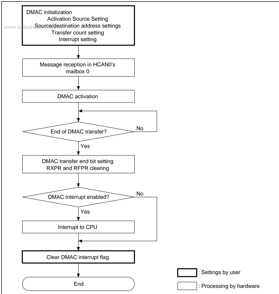
Figure 16.15 DMAC Transfer Flowchart
