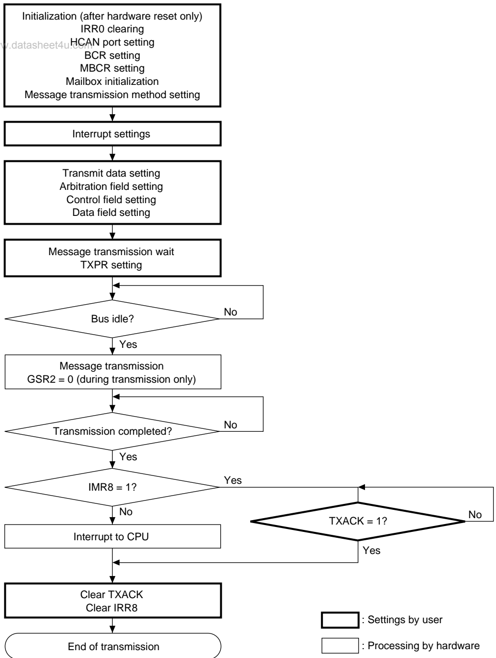
Figure 16.9 Transmission Flowchart
