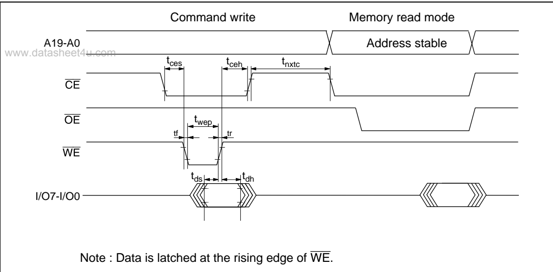
Figure 22.32 Memory Read Timing after Command Write
