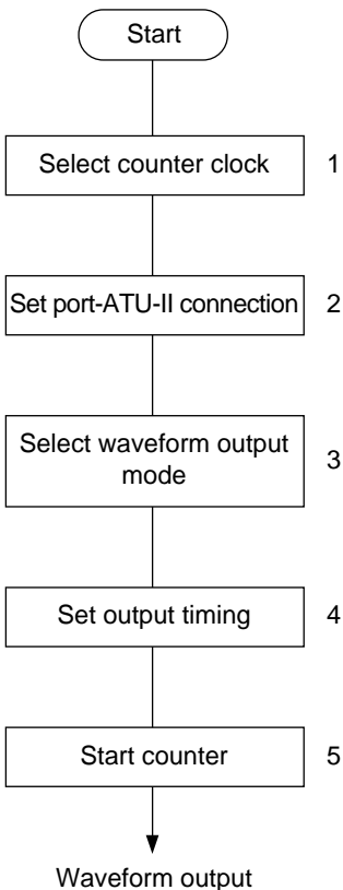
Figure 11.54 Sample Setup Procedure for Waveform Output by Output Compare-Match
