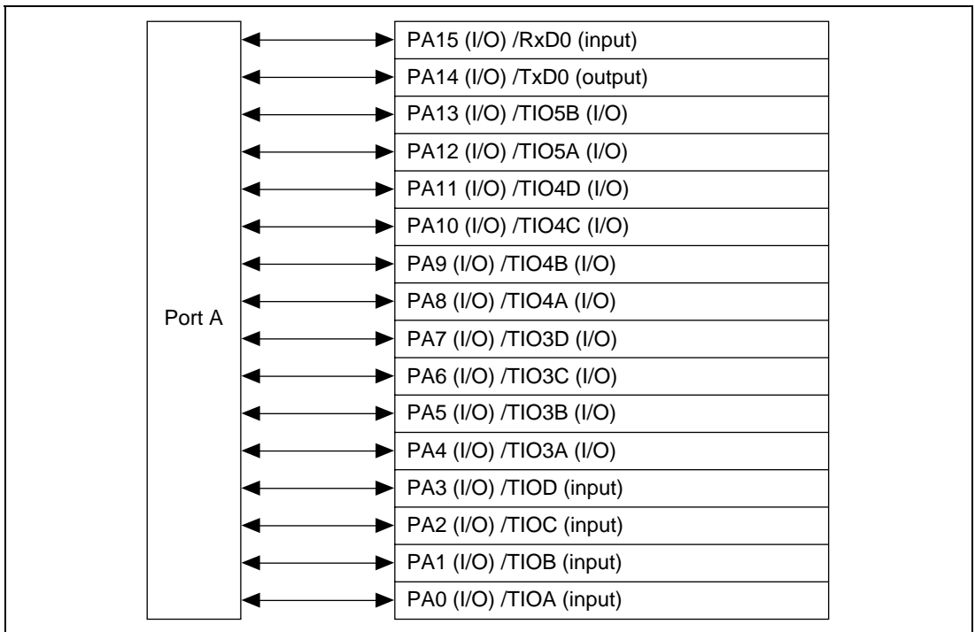
Figure 21.1 Port A
