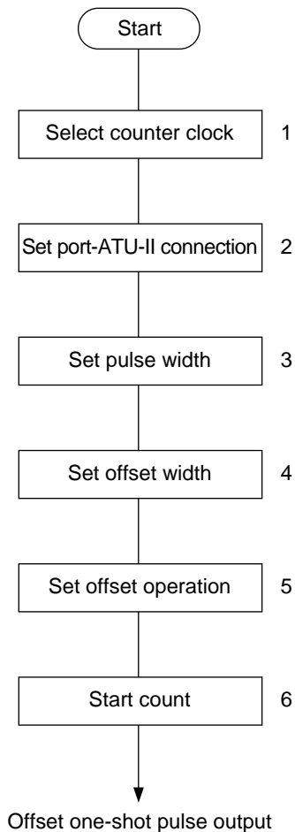
Figure 11.57 Sample Setup Procedure for Offset One-Shot Pulse Output
