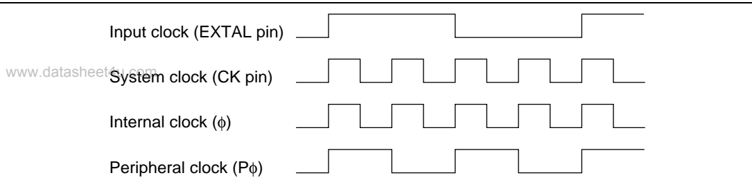
Figure 5.2 Input Clock and System Clock
