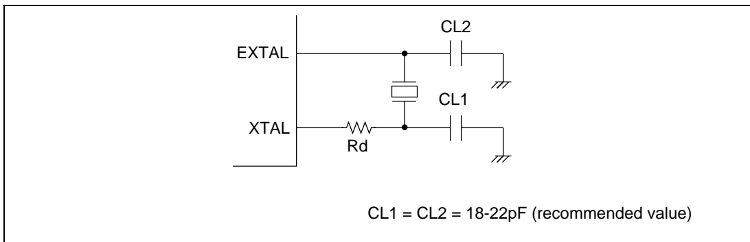
Figure 5.3 Connection of Crystal Oscillator (Example)
