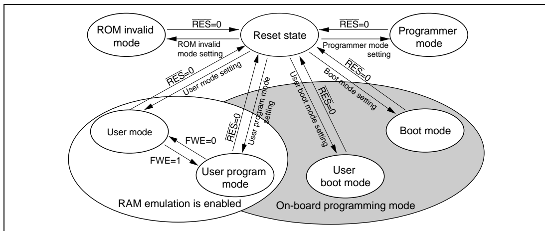
Figure 22.2 Mode Transition of Flash Memory
