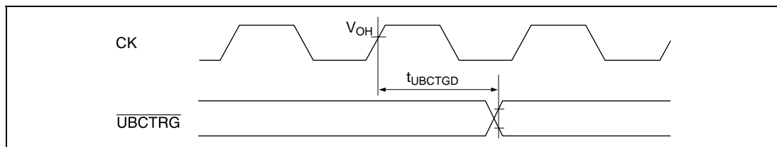
Figure 26.27 UBC Trigger Timing
