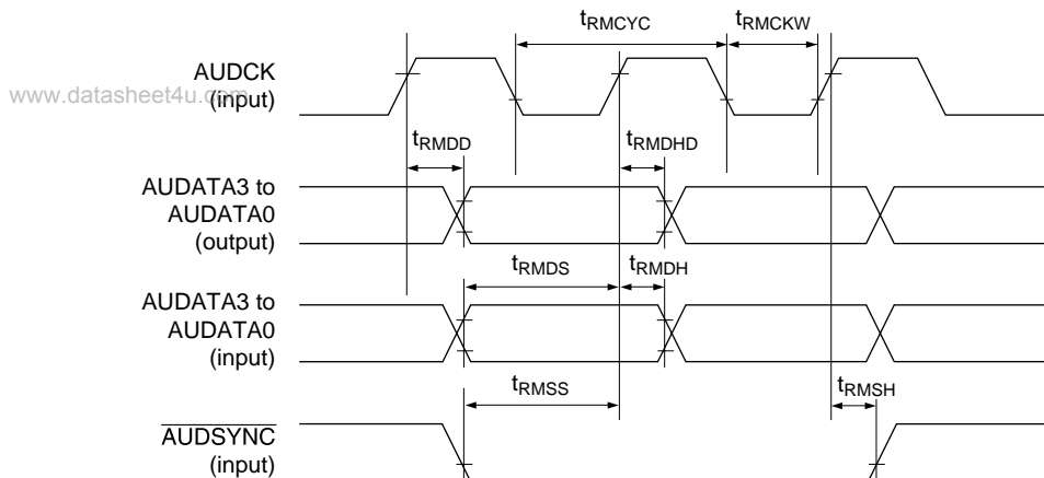
Figure 26.26 RAM Monitor Timing
