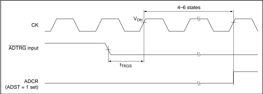
Figure 26.19 External Trigger Input Timing
