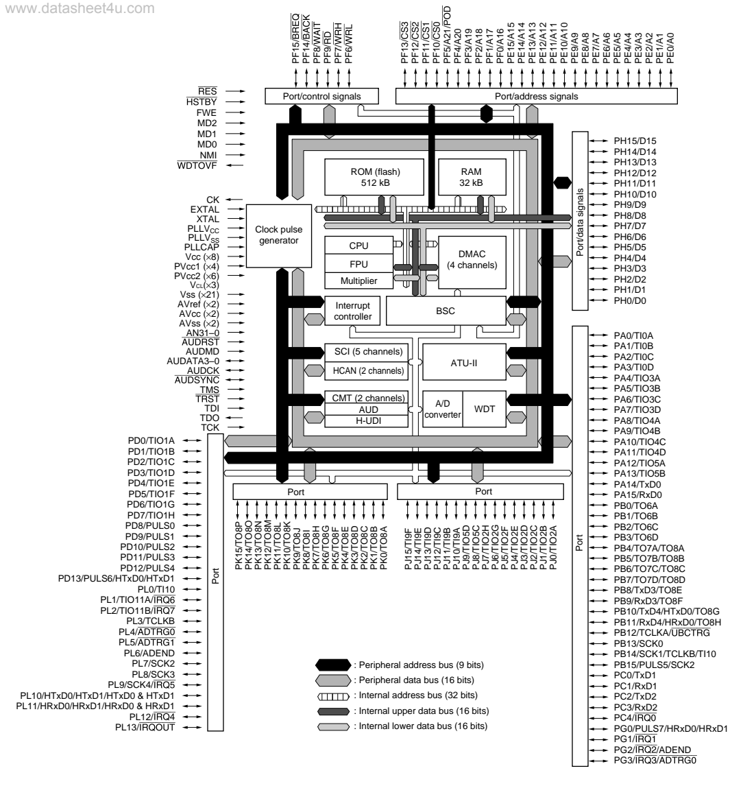
Figure 1.1 Block Diagram
