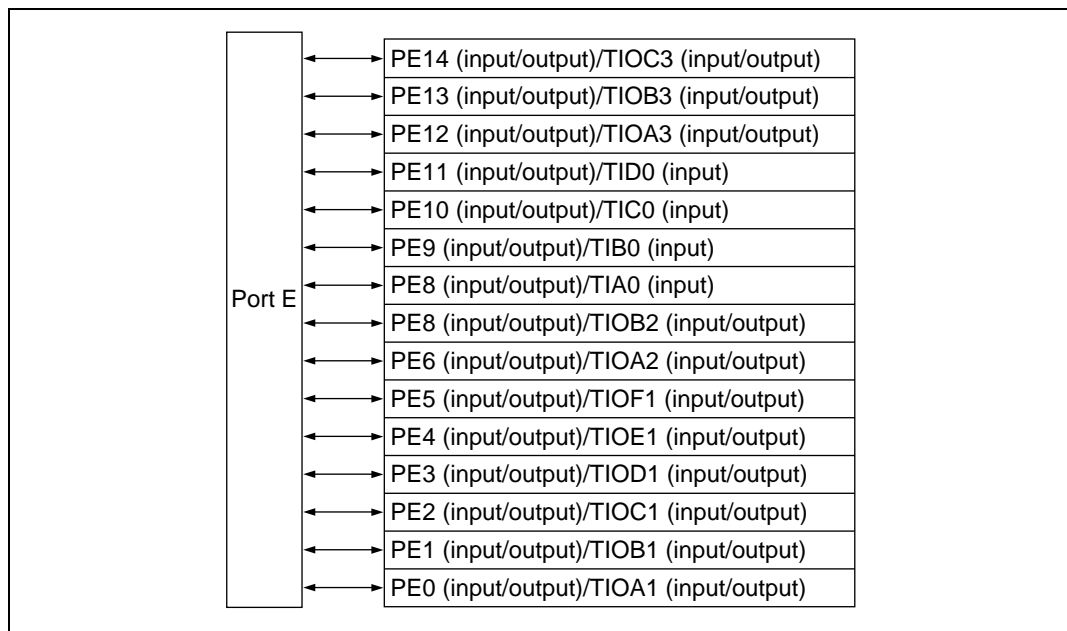
Figure 17.5 Port E
