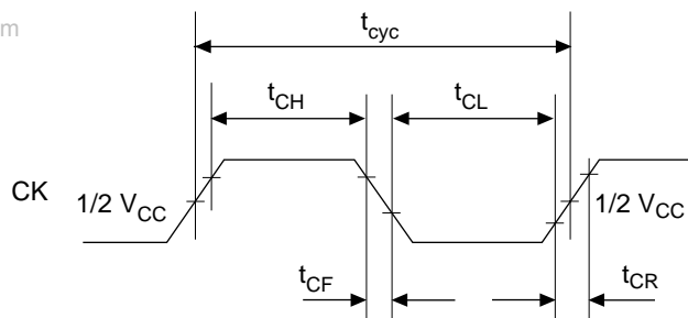
Figure 22.1 System Clock Timing
