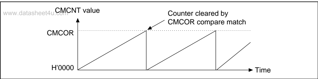
Figure 15.2 Counter Operation
