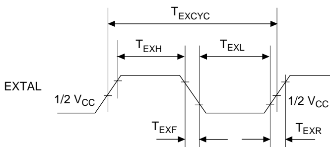
Figure 22.2 EXTAL Clock Input Timing
