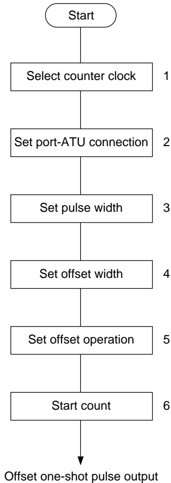
Figure 10.49 Sample Setup Procedure for Offset One-Shot Pulse Output
