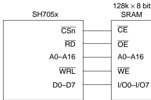
Figure 8.12 8-Bit Data Bus Width SRAM Connection
