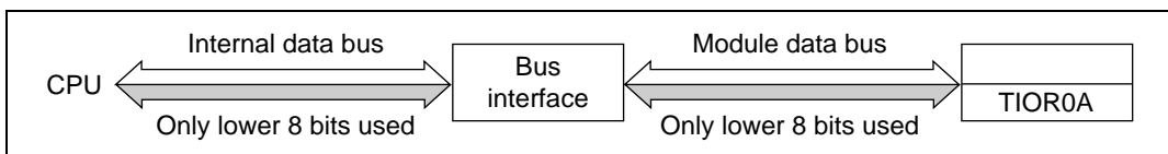
Figure 10.44 Byte Read/Write Access to TIORA
