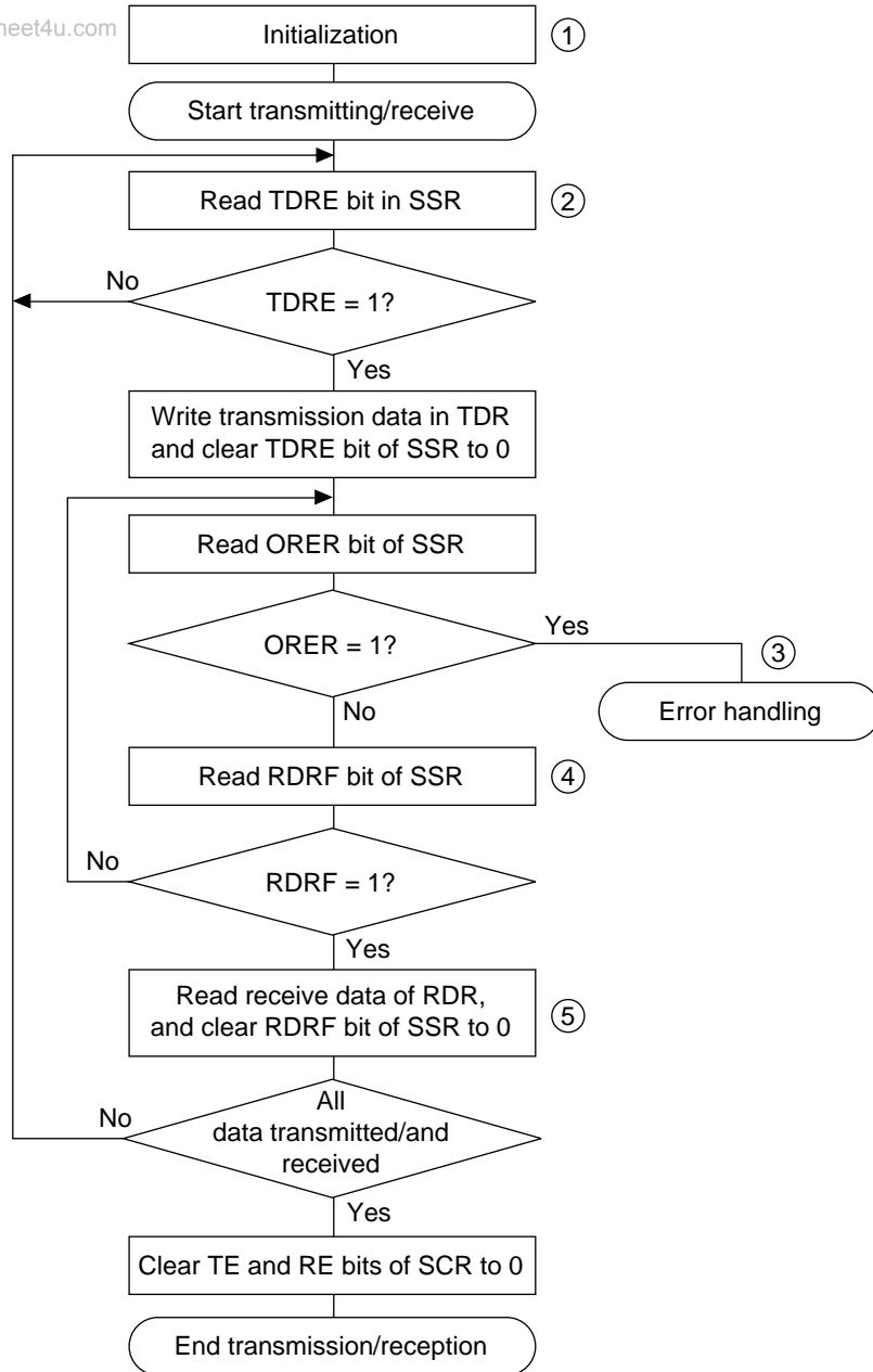
Figure 13.22 Sample Flowchart for Serial Transmission
