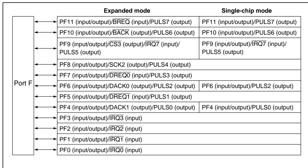
Figure 17.6 Port F
