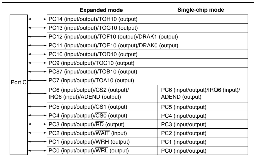
Figure 17.3 Port C
