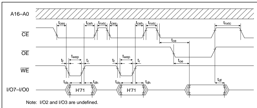
Figure 19.20 Status Read Mode Timing Waveforms
