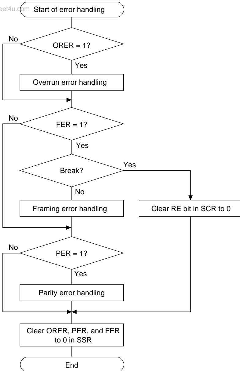
Figure 13.8 Sample Flowchart for Receiving Serial Data (2)
