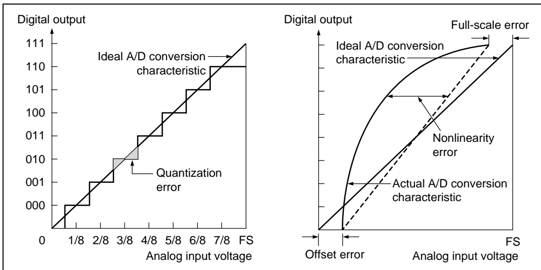
Figure 14.9 A/D Conversion Precision Definitions
