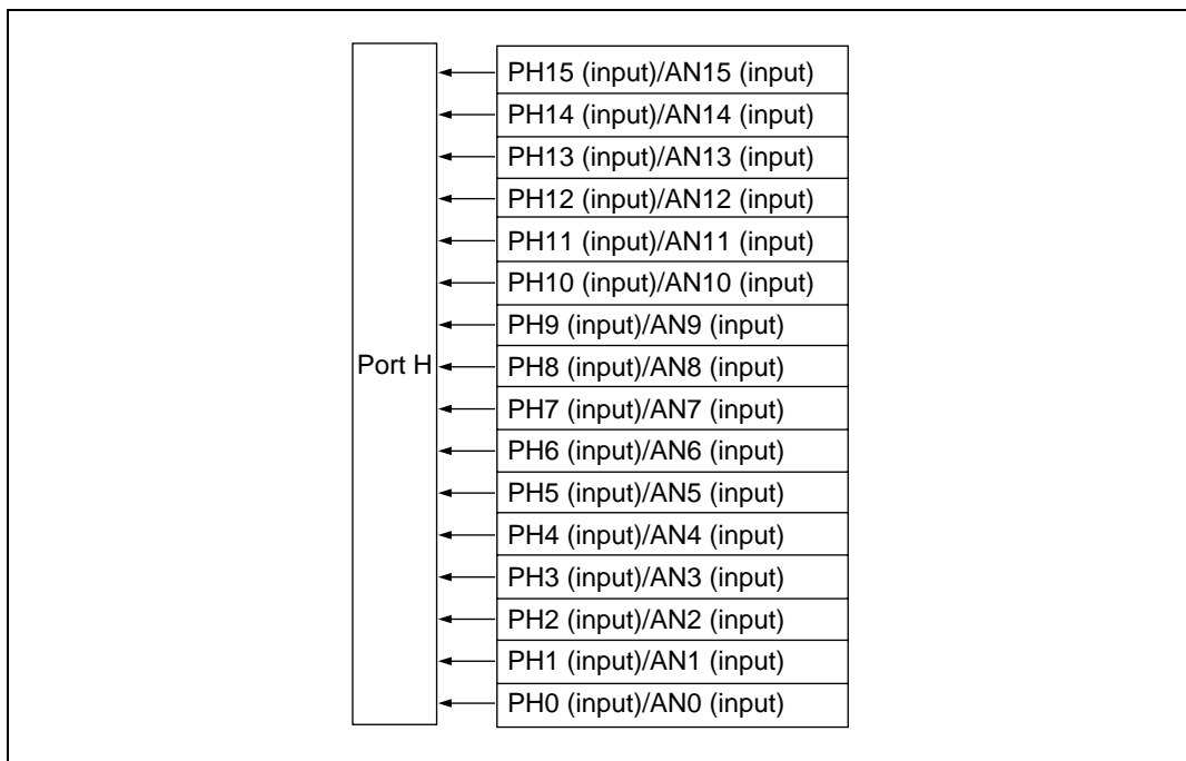
Figure 17.8 Port H
