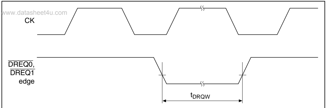
Figure 22.12 DREQ0 and DREQ1 Input Timing (2)
