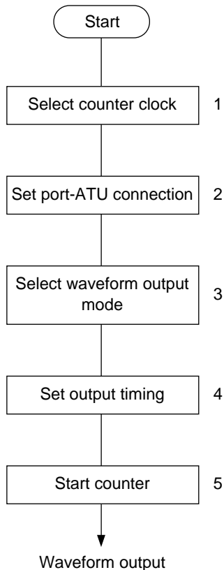
Figure 10.46 Sample Setup Procedure for Waveform Output by Output Compare-Match
