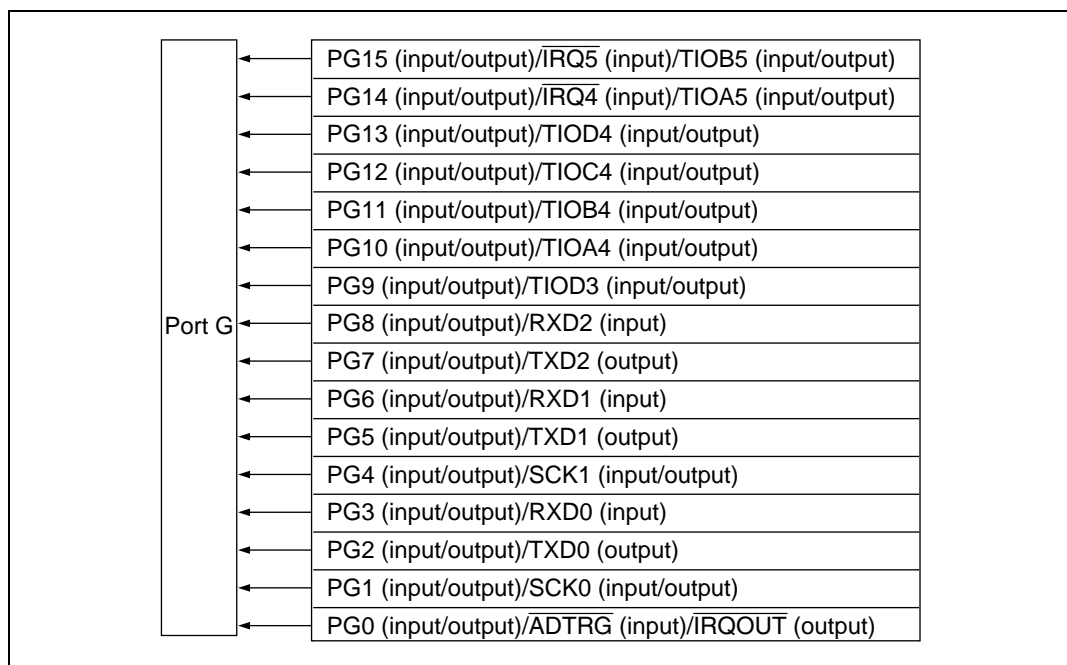
Figure 17.7 Port G
