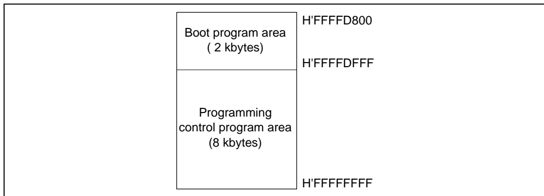
Figure 19.5 RAM Areas in Boot Mode
