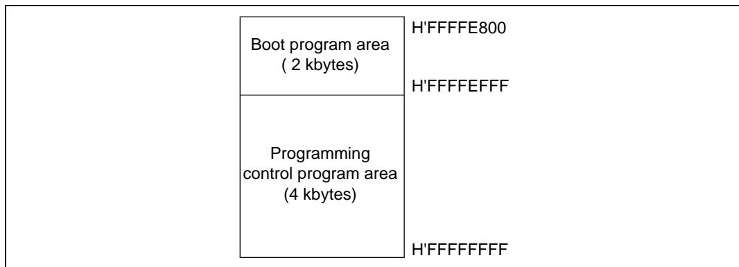
Figure 18.5 RAM Areas in Boot Mode
