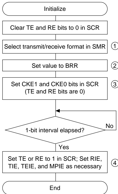
Figure 13.4 Sample Flowchart for SCI Initialization
