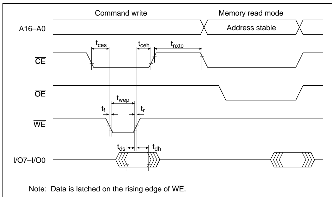
Figure 19.14 Timing Waveforms for Memory Read after Memory Write
