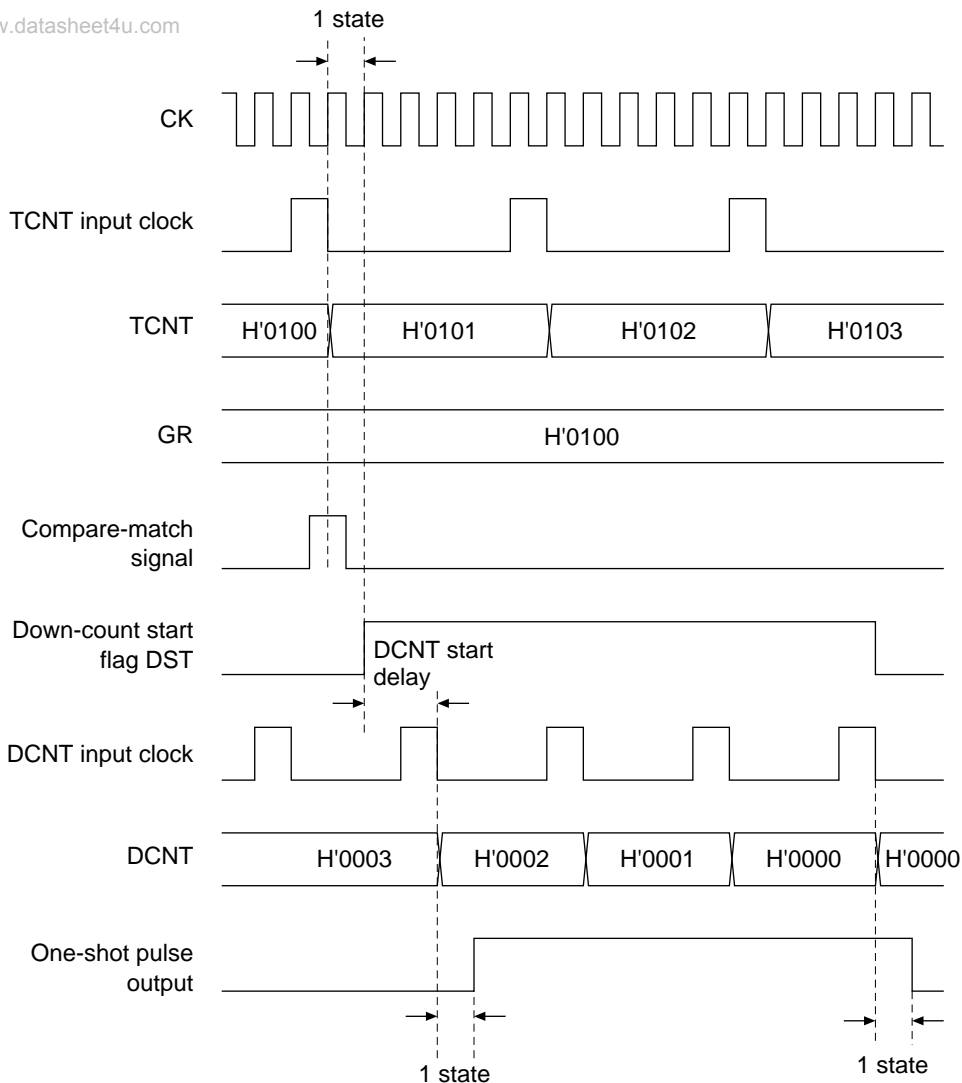
Figure 10.24 Offset One-Shot Pulse Function Pulse Output Timing
