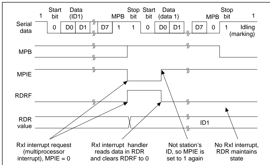
Figure 13.14 SCI Receive Operation (ID Does Not Match)
