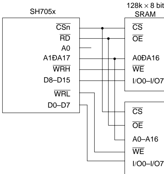
Figure 8.13 16-Bit Data Bus Width SRAM Connection
