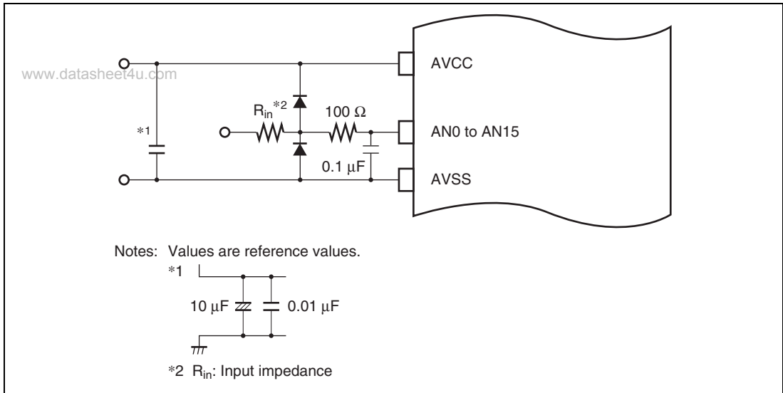
Figure 13.7 Example of Analog Input Protection Circuit
