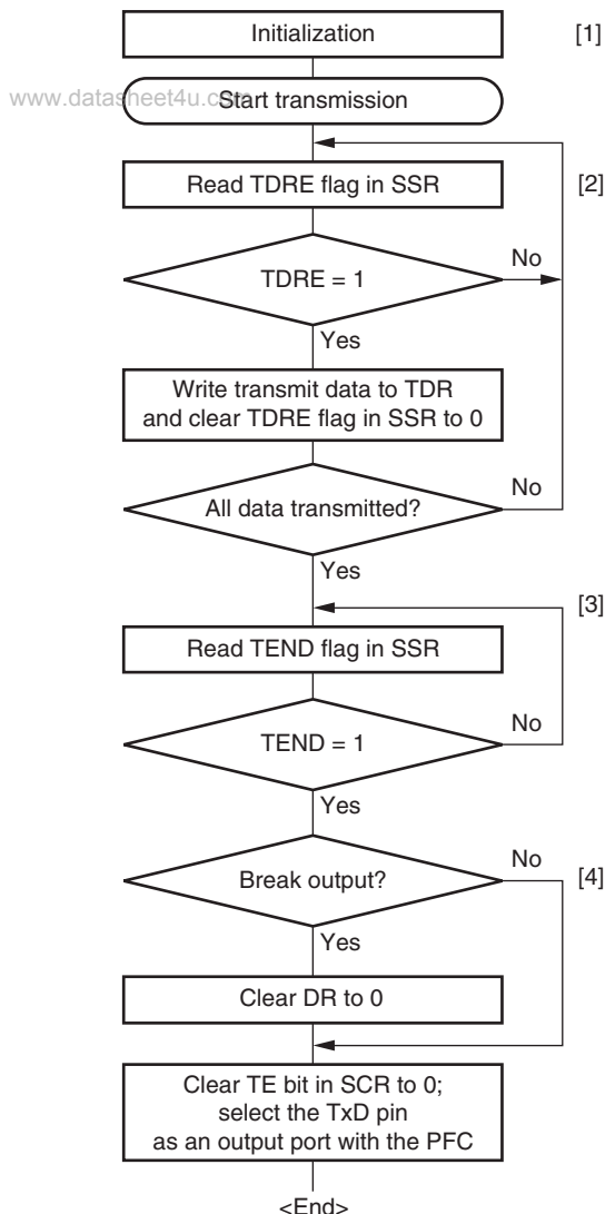
Figure 12.7 Sample Serial Transmission Flowchart
