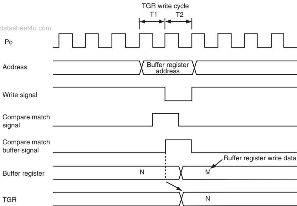
Figure 10.75 Contention between Buffer Register Write and Compare Match (Channels 3 and 4)
