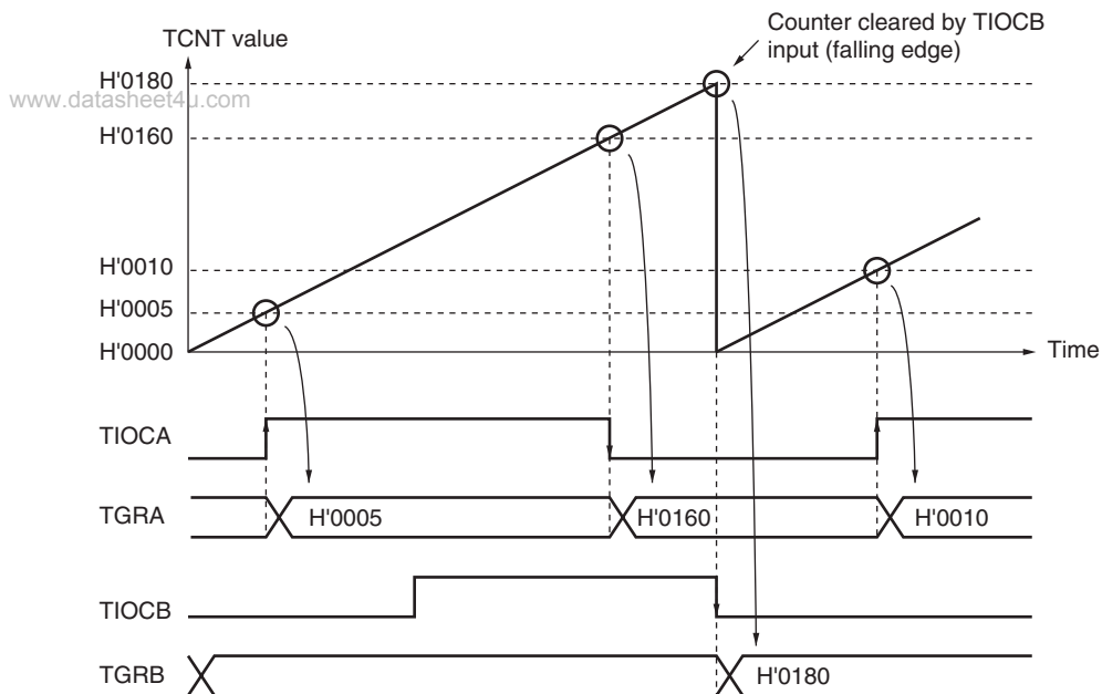
Figure 10.10 Example of Input Capture Operation
