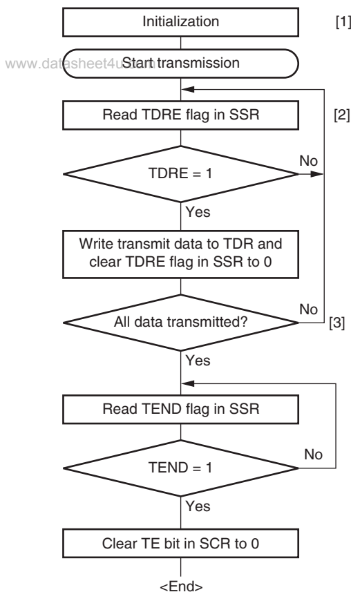
Figure 12.17 Sample Serial Transmission Flowchart
