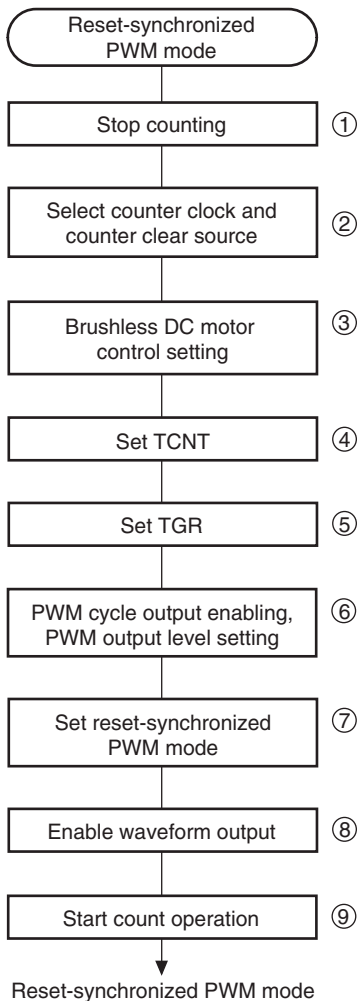
Figure 10.30 Procedure for Selecting the Reset-Synchronized PWM Mode
