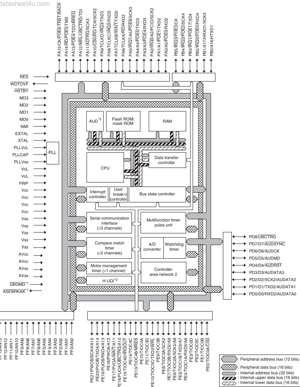
Figure 1.1 Block Diagram of SH7047
