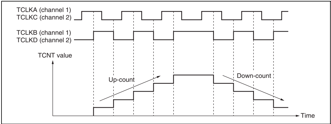
Figure 10.28 Example of Phase Counting Mode 4 Operation
