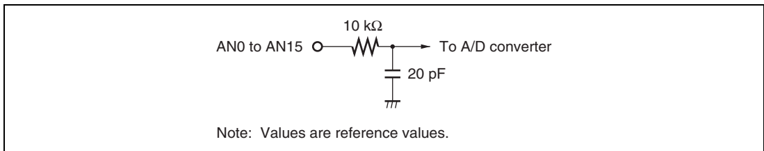
Figure 13.8 Analog Input Pin Equivalent Circuit
