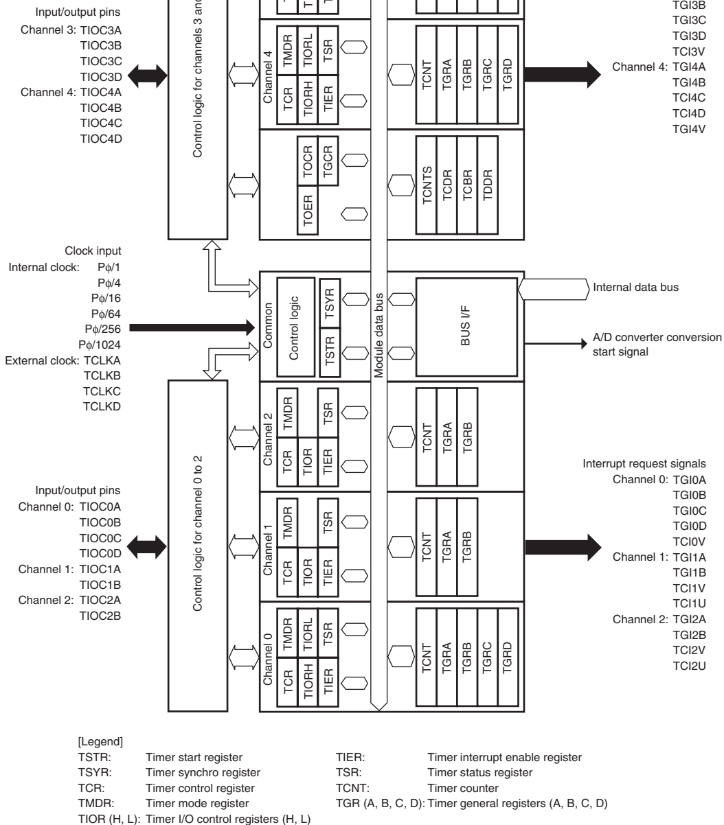
Figure 10.1 Block Diagram of MTU
