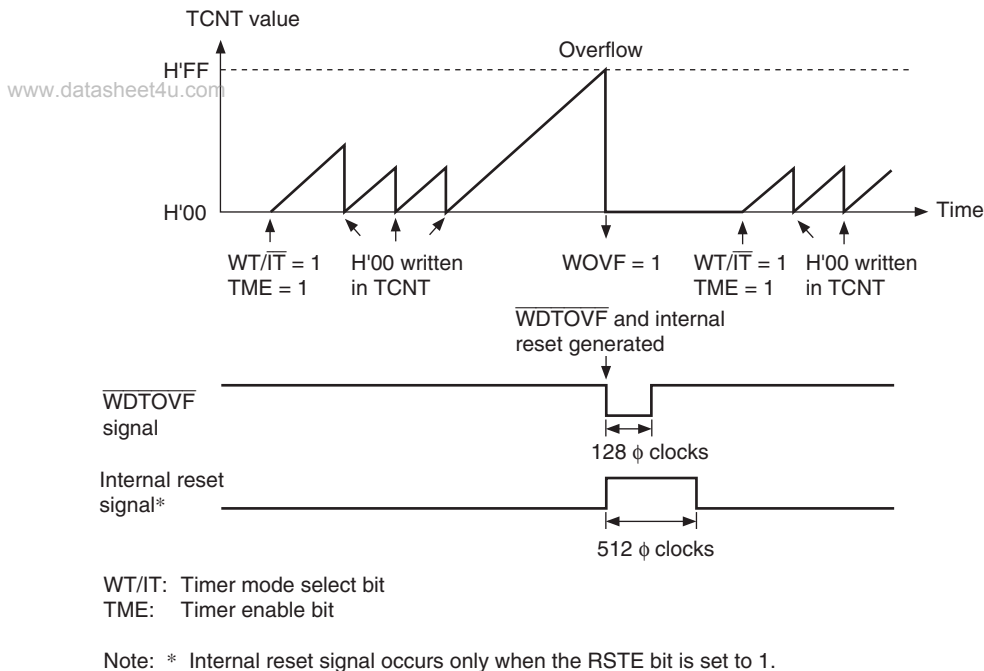
Figure 11.2 Operation in Watchdog Timer Mode
