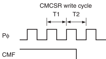
Figure 14.5 Timing of CMF Clear by the CPU
