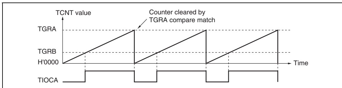
Figure 10.21 Example of PWM Mode Operation
