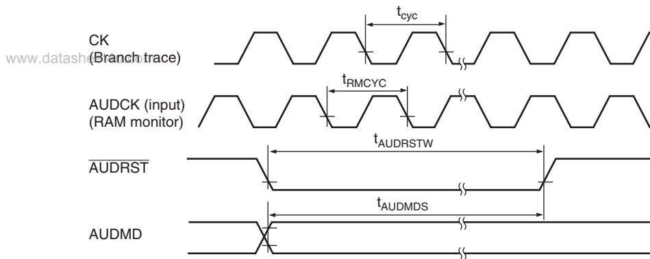
Figure 25.26 AUD Reset Timing
