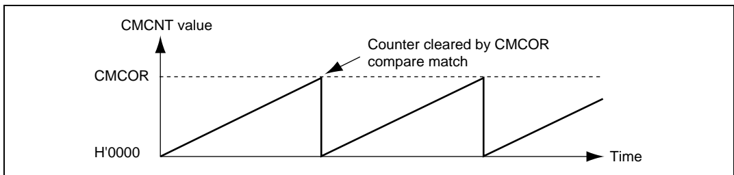
Figure 14.2 Counter Operation
