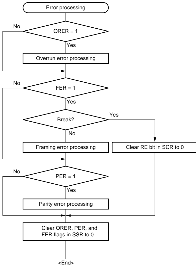
Figure 12.9 Sample Serial Reception Data Flowchart (2)
