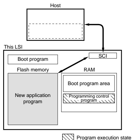
Figure 18.3 Boot Mode
