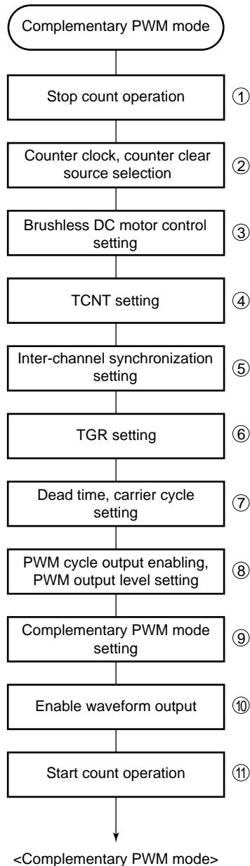
Figure 10.33 Example of Complementary PWM Mode Setting Procedure
