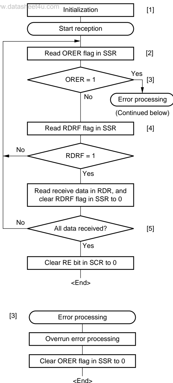
Figure 12.19 Sample Serial Reception Flowchart
