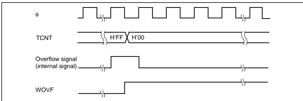
Figure 11.5 Timing of Setting WOVF
