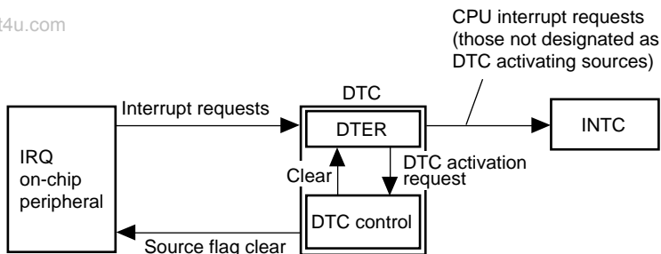
Figure 8.2 Activating Source Control Block Diagram
