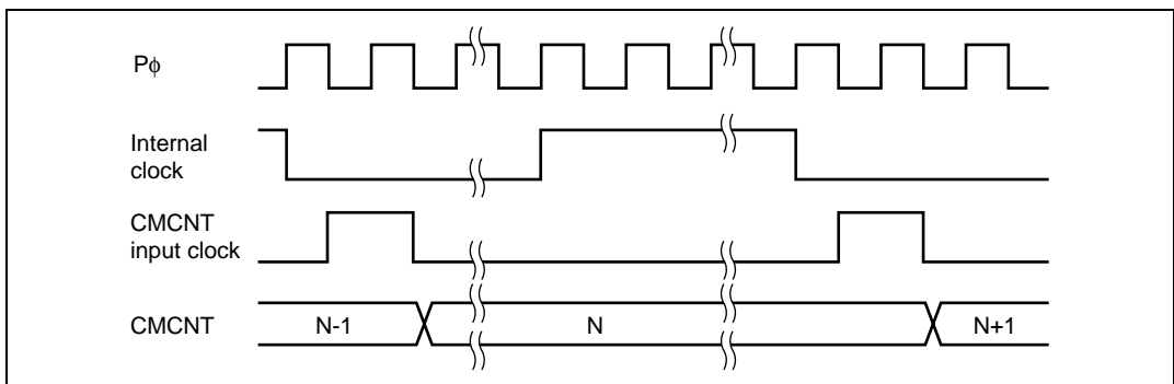
Figure 14.3 Count Timing
