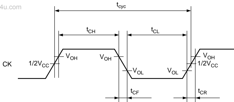
Figure 22.2 System Clock Timing
